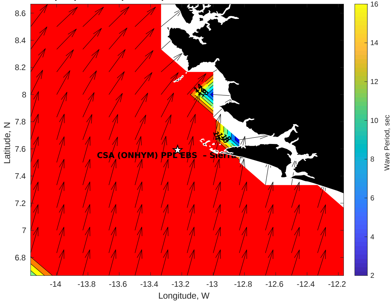
GFS Wave Period (sec) for CSA (ONHYM) PPL EBS - Sierra Leone at 14-Dec-2025 09:00:00
