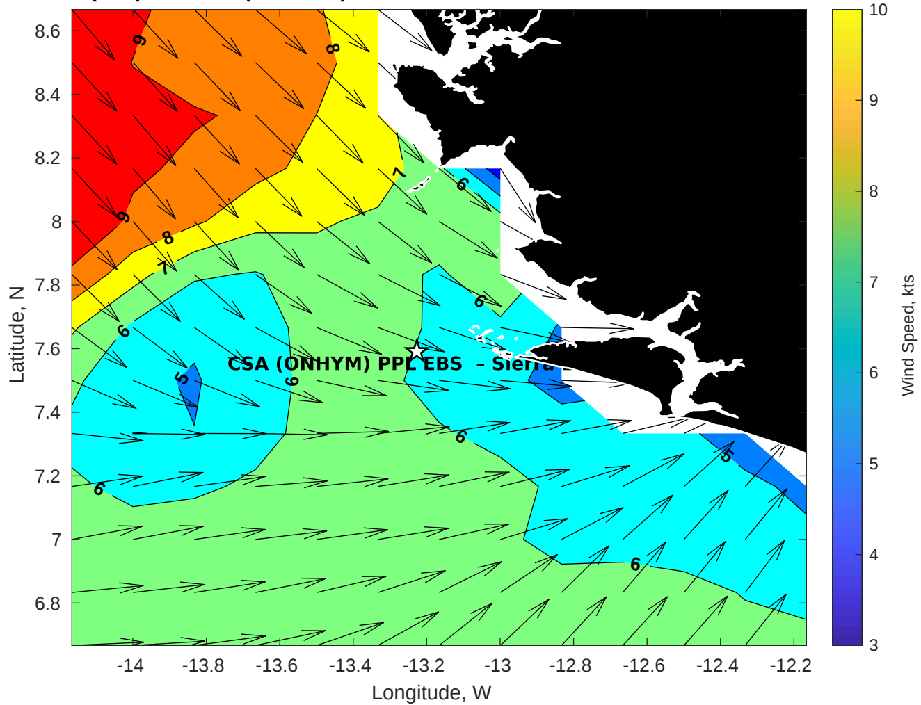
GFS Winds (kts) for CSA (ONHYM) PPL EBS - Sierra Leone at 14-Dec-2025 09:00:00
