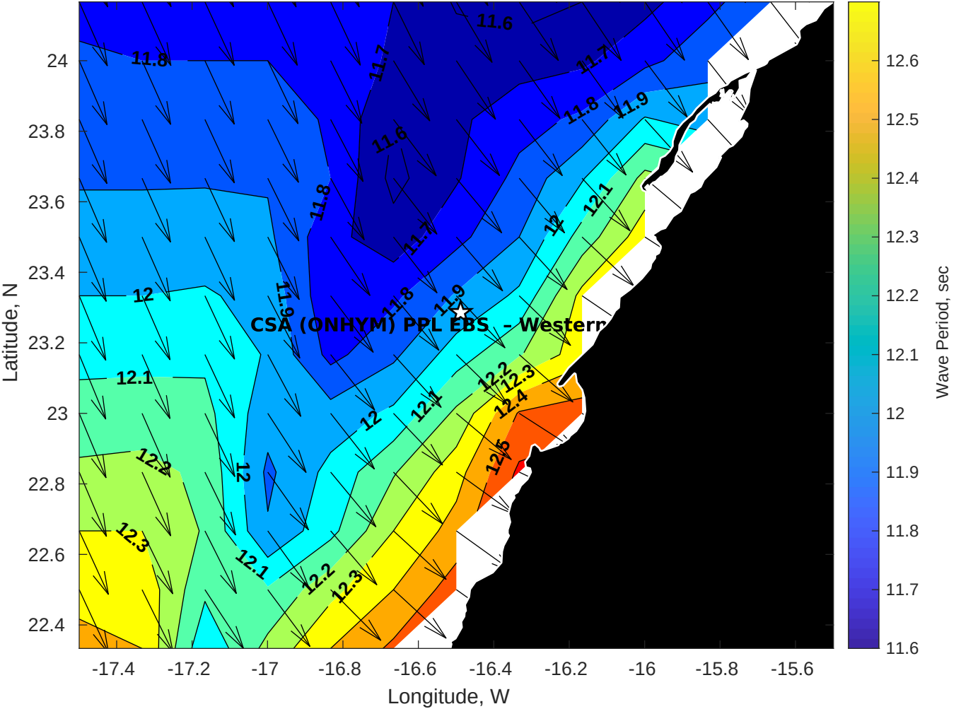
GFS Wave Period (sec) for CSA (ONHYM) PPL EBS - Western Sahara at 14-Dec-2025 09:00:00
