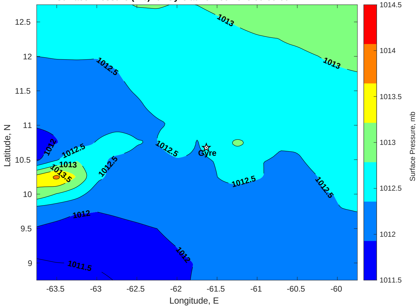
Surface Pressure (mb) for Gyre at 16-Dec-2025 00:00:00
