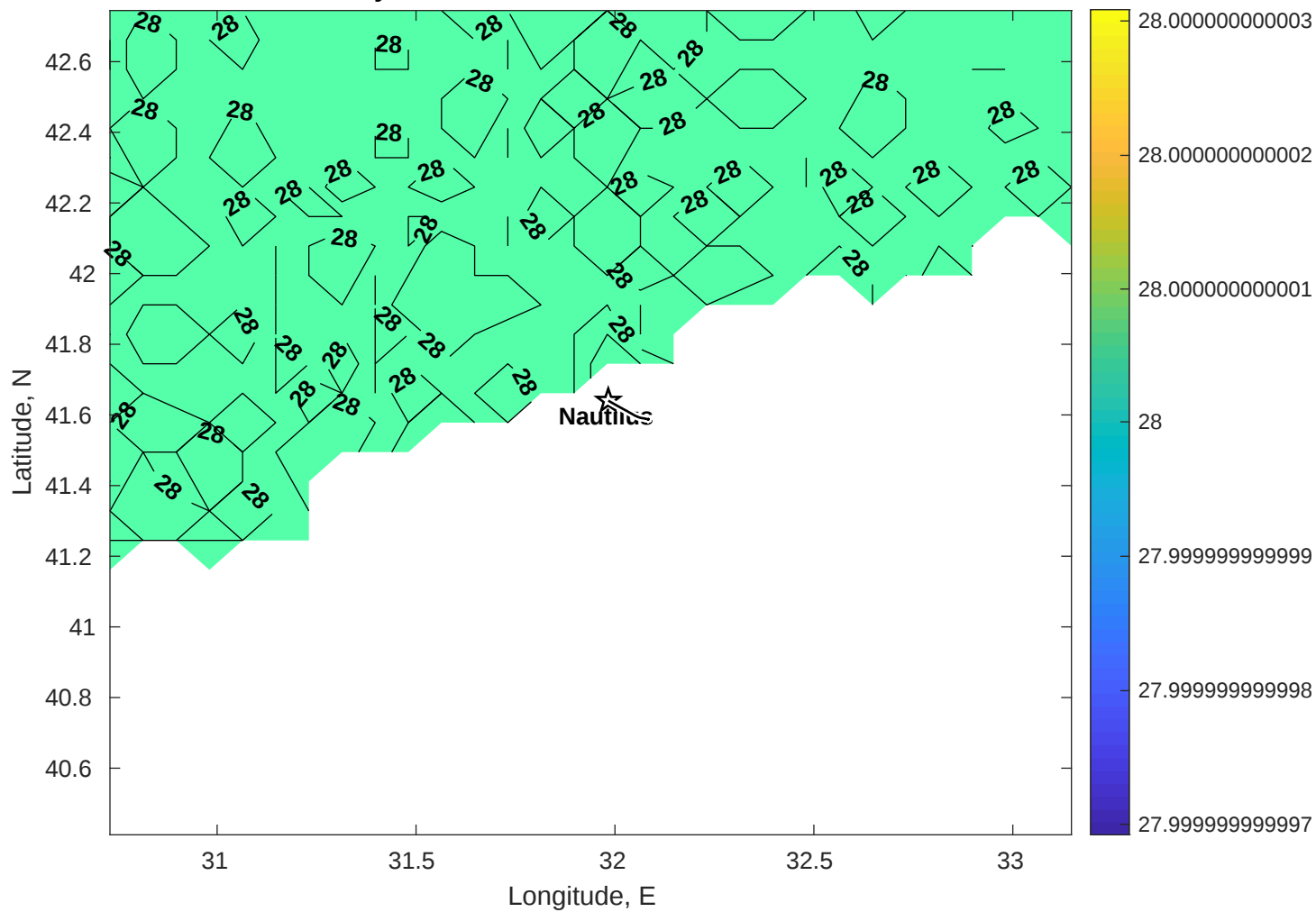
Surface Salinity for Nautilus at 13-Dec-2025 00:00:00
