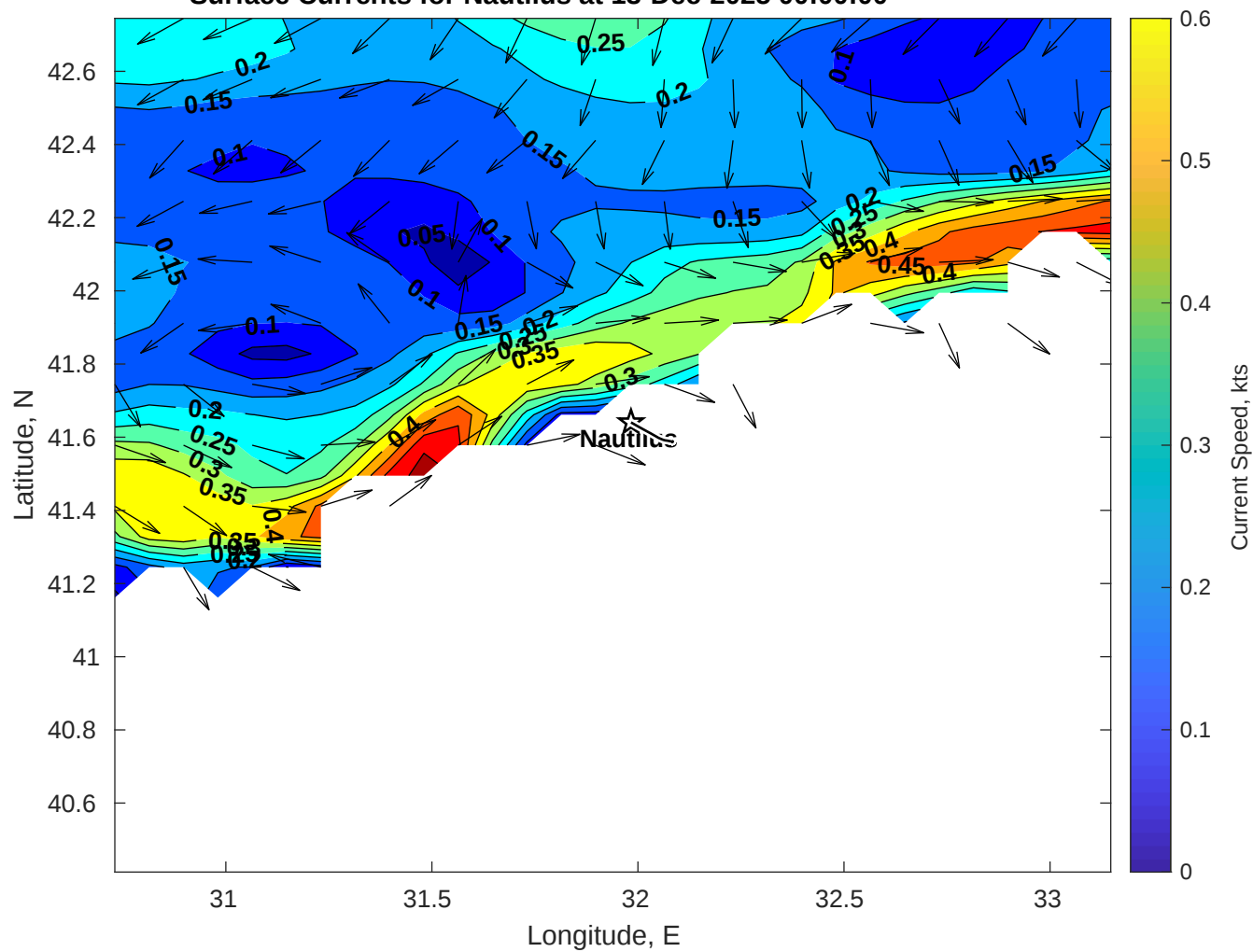
Surface Currents for Nautilus at 13-Dec-2025 00:00:00
