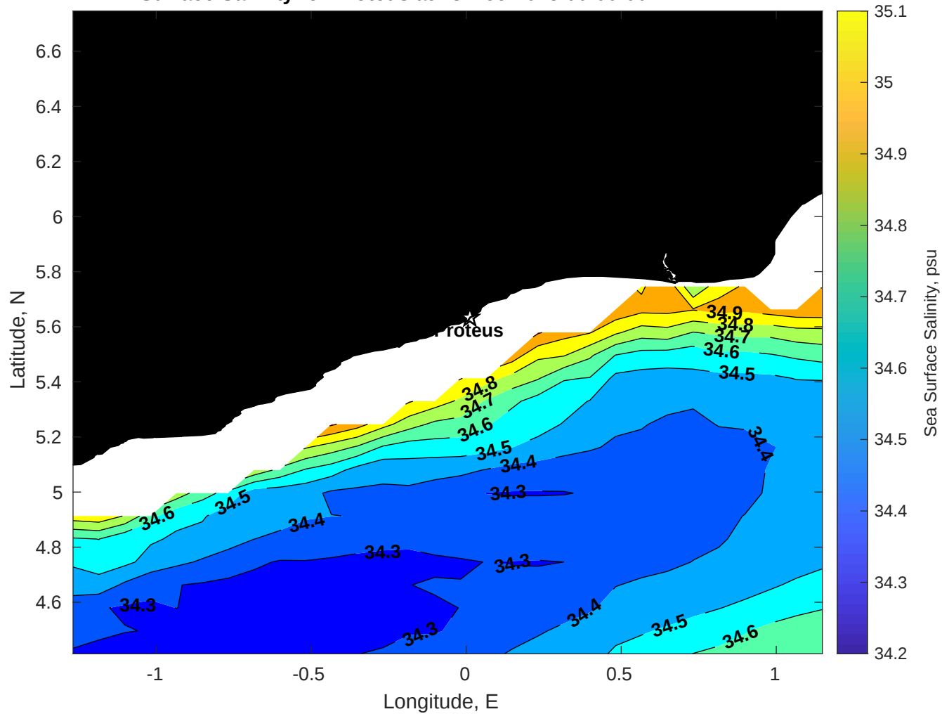
Surface Salinity for Proteus at 13-Dec-2025 00:00:00
