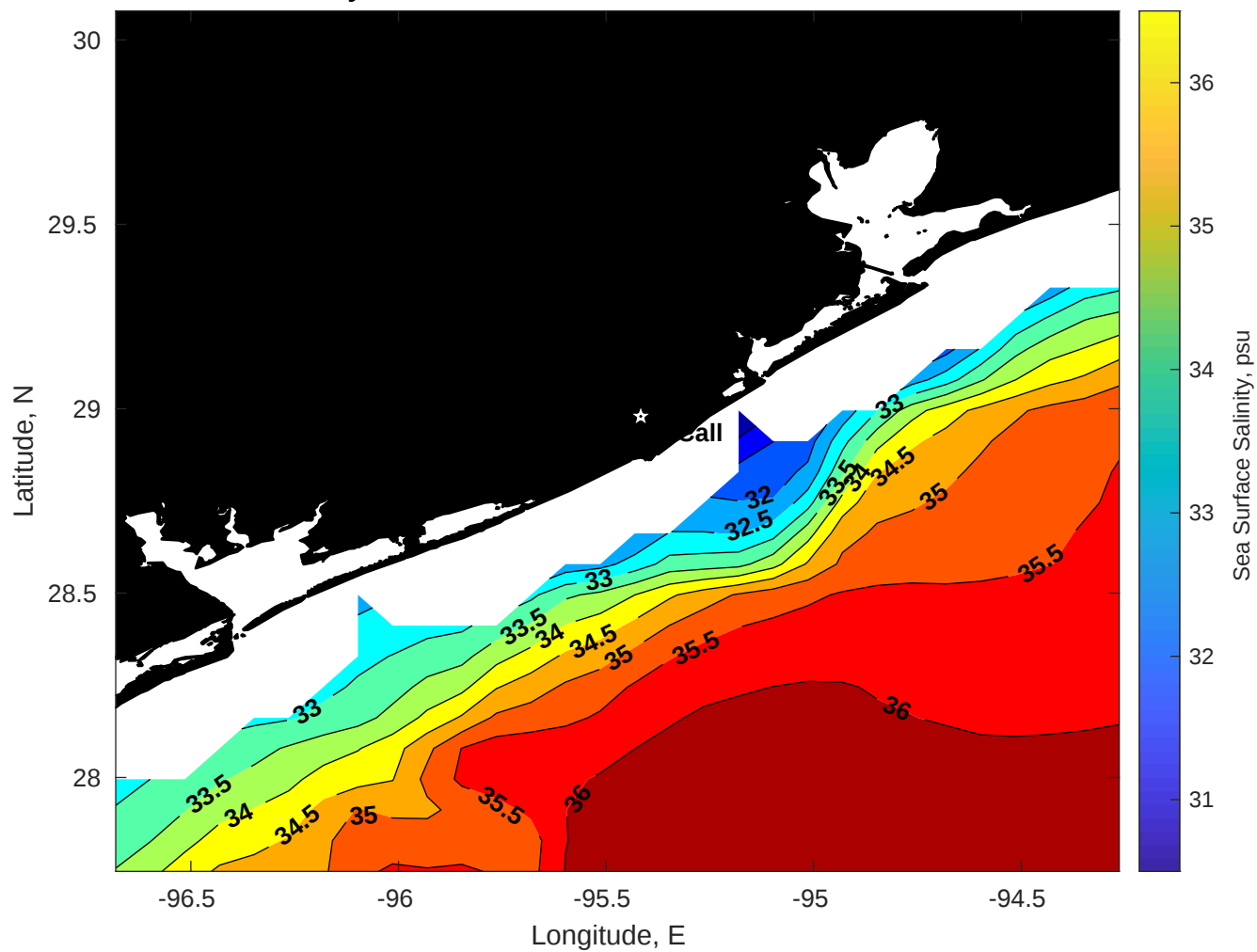
Surface Salinity for Brooks McCall at 14-Dec-2025 00:00:00
