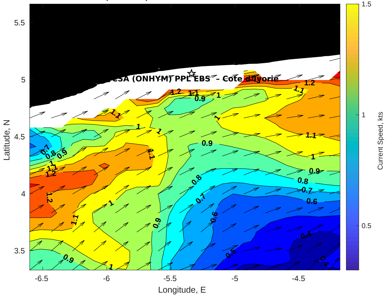
Surface Currents for CSA (ONHYM) PPL EBS - Cote d'Ivoire at 14-Dec-2025 00:00:00
