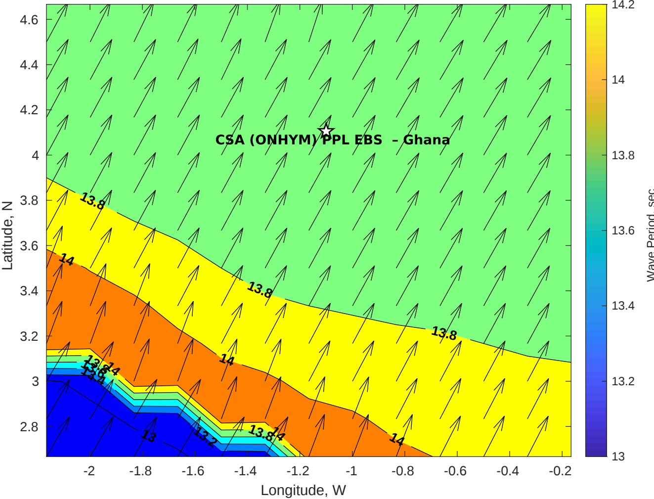
GFS Wave Period (sec) for CSA (ONHYM) PPL EBS - Ghana at 15-Dec-2025 09:00:00
