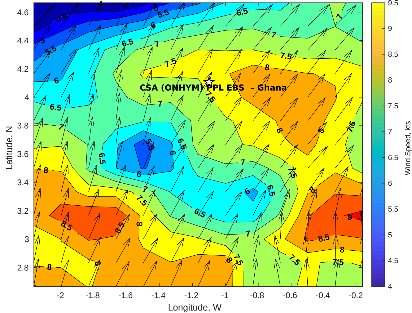
GFS Winds (kts) for CSA (ONHYM) PPL EBS - Ghana at 15-Dec-2025 09:00:00
