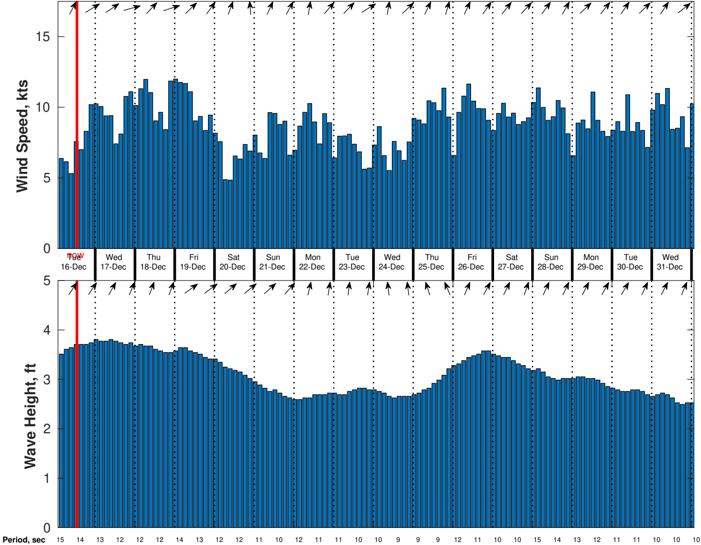
Wind & Wave Forecast for CSA (ONHYM) PPL EBS - Ghana from 15-Dec-2025 02:00:00 to 31-Dec-2025 02:00:00
