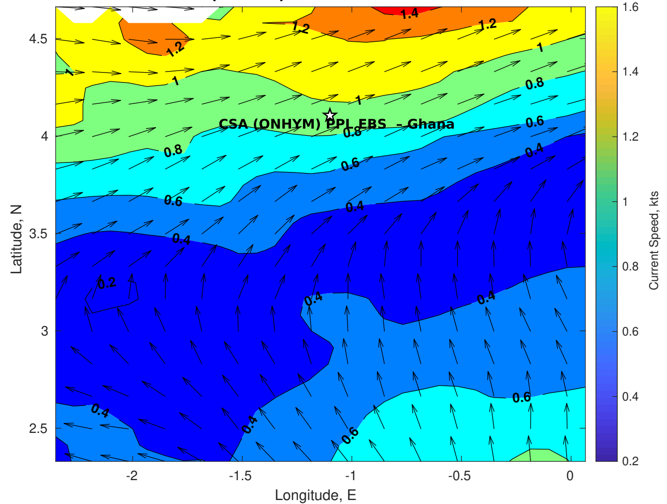
Surface Currents for CSA (ONHYM) PPL EBS - Ghana at 14-Dec-2025 00:00:00
