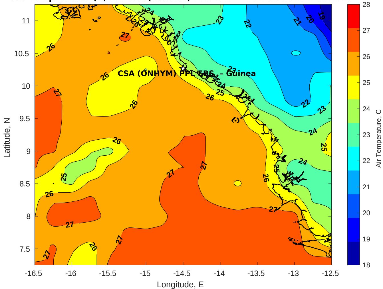
Air Temperature (C) for CSA (ONHYM) PPL EBS - Guinea at 15-Dec-2025
