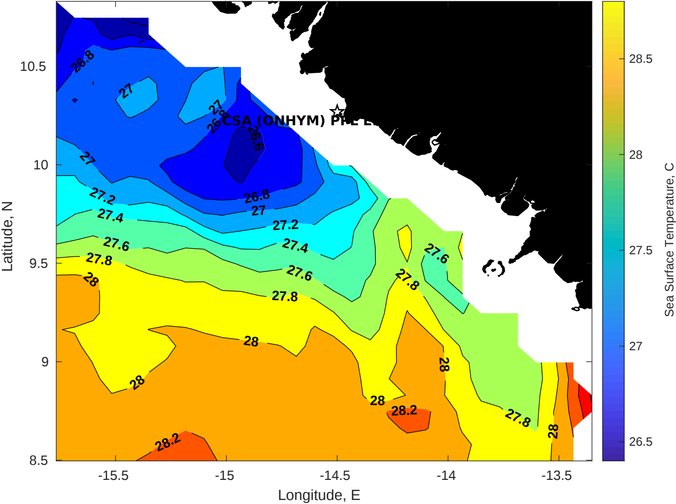
SST for CSA (ONHYM) PPL EBS - Guinea at 14-Dec-2025 00:00:00
