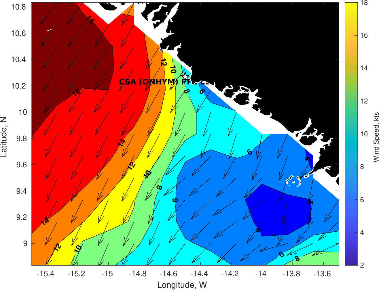
GFS Winds (kts) for CSA (ONHYM) PPL EBS - Guinea at 15-Dec-2025 09:00:00
