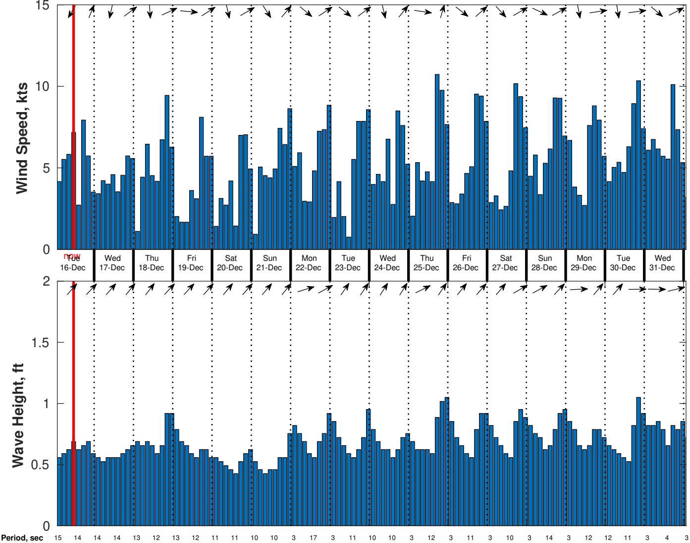
Wind & Wave Forecast for CSA (ONHYM) PPL EBS - Guinea from 15-Dec-2025 01:00:00 to 31-Dec-2025 01:00:00
