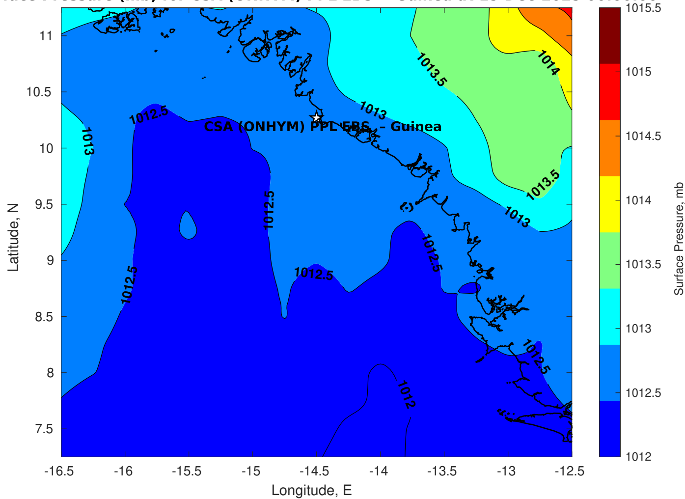
Surface Pressure (mb) for CSA (ONHYM) PPL EBS - Guinea at 15-Dec-2025 00:00:00
