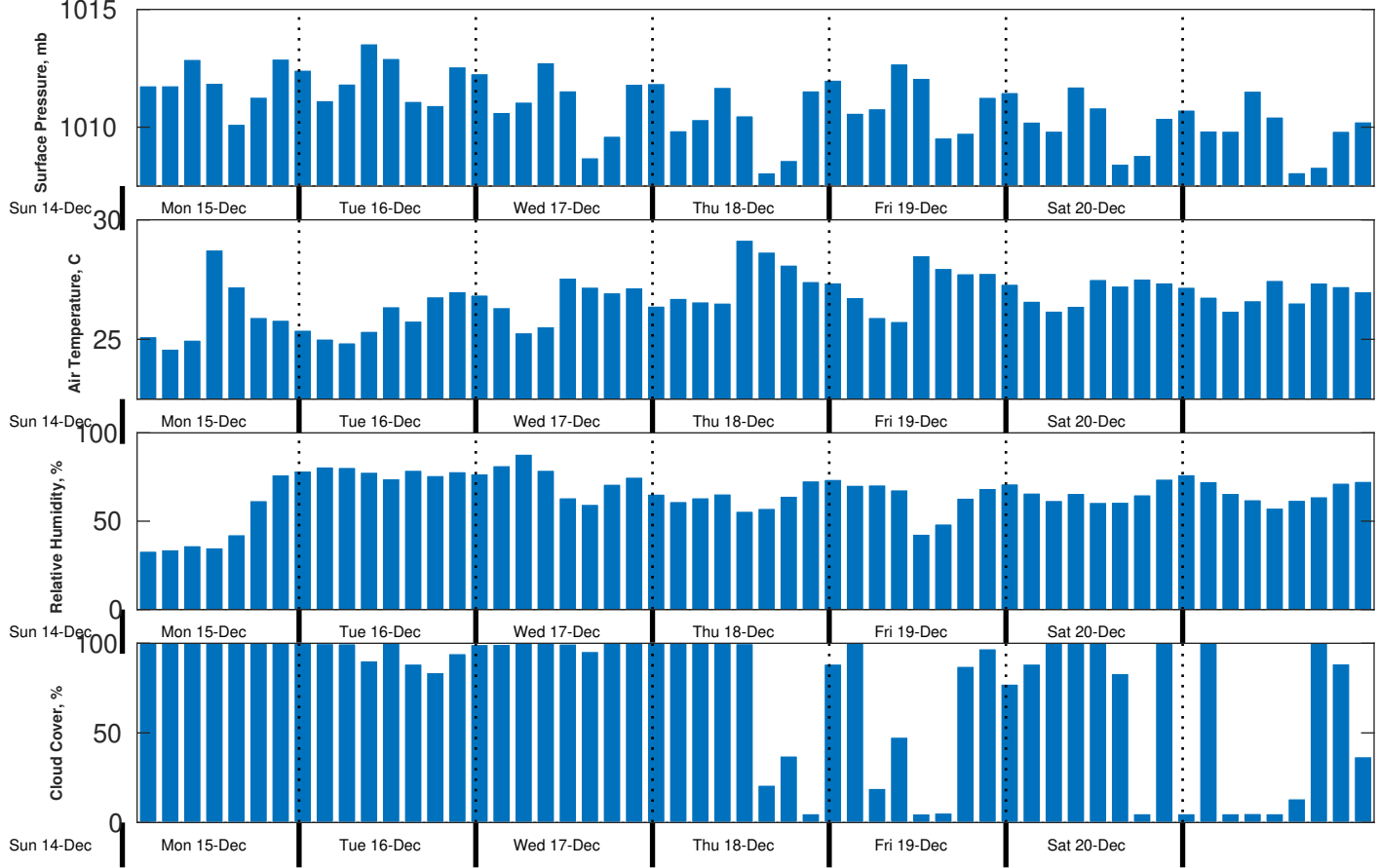
Met Forecast for CSA (ONHYM) PPL EBS - Guinea from 15-Dec-2025 00:00:00 to 22-Dec-2025 00:00:00
