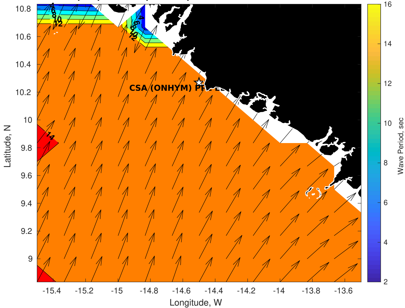
GFS Wave Period (sec) for CSA (ONHYM) PPL EBS - Guinea at 15-Dec-2025 09:00:00
