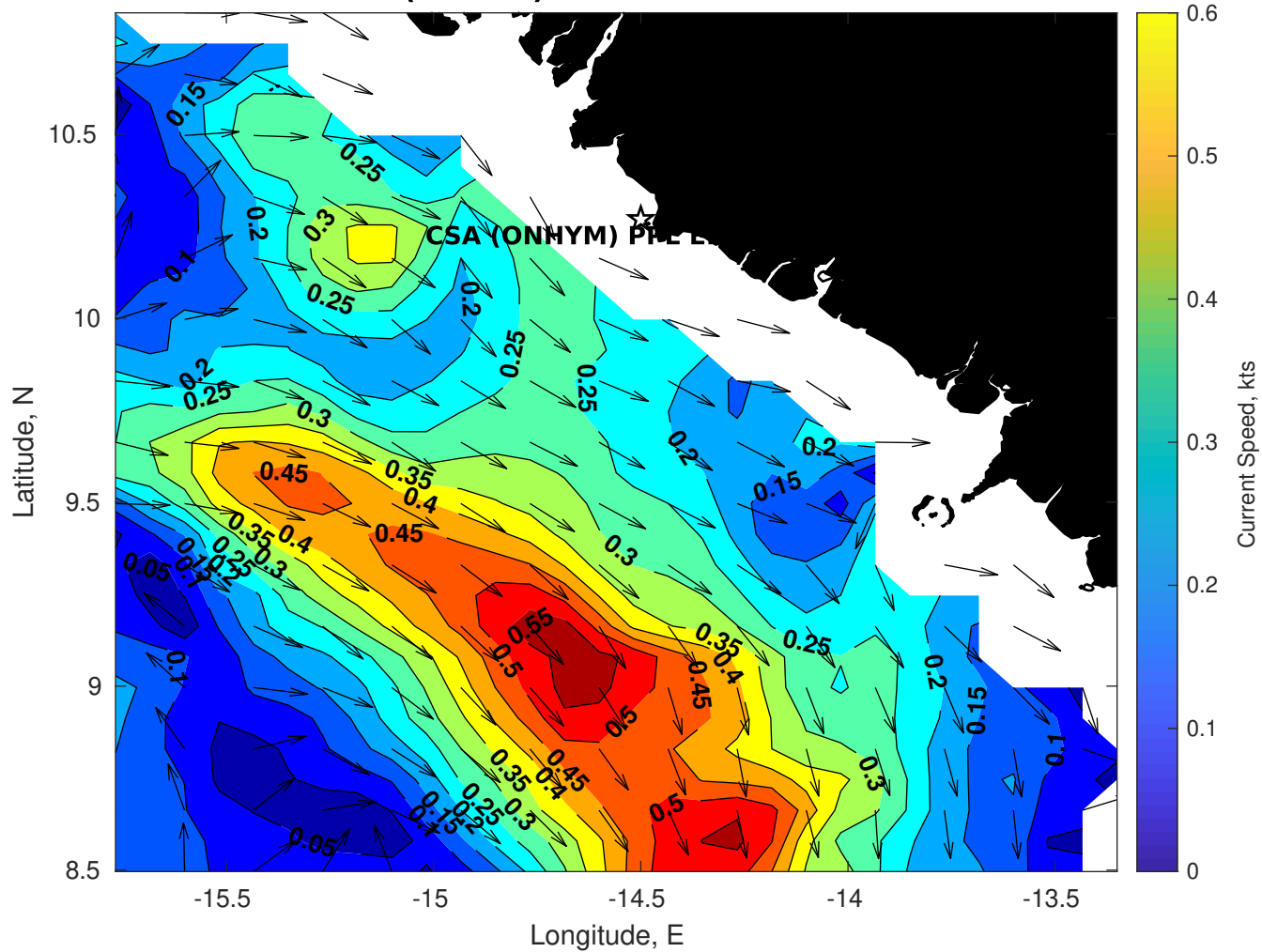
Surface Currents for CSA (ONHYM) PPL EBS - Guinea at 14-Dec-2025 00:00:00
