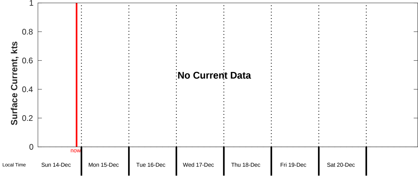
Surface Current Forecast for CSA (ONHYM) PPL EBS - Guinea from 14-Dec-2025 00:00:00 to 22-Dec-2025 00:00:00
