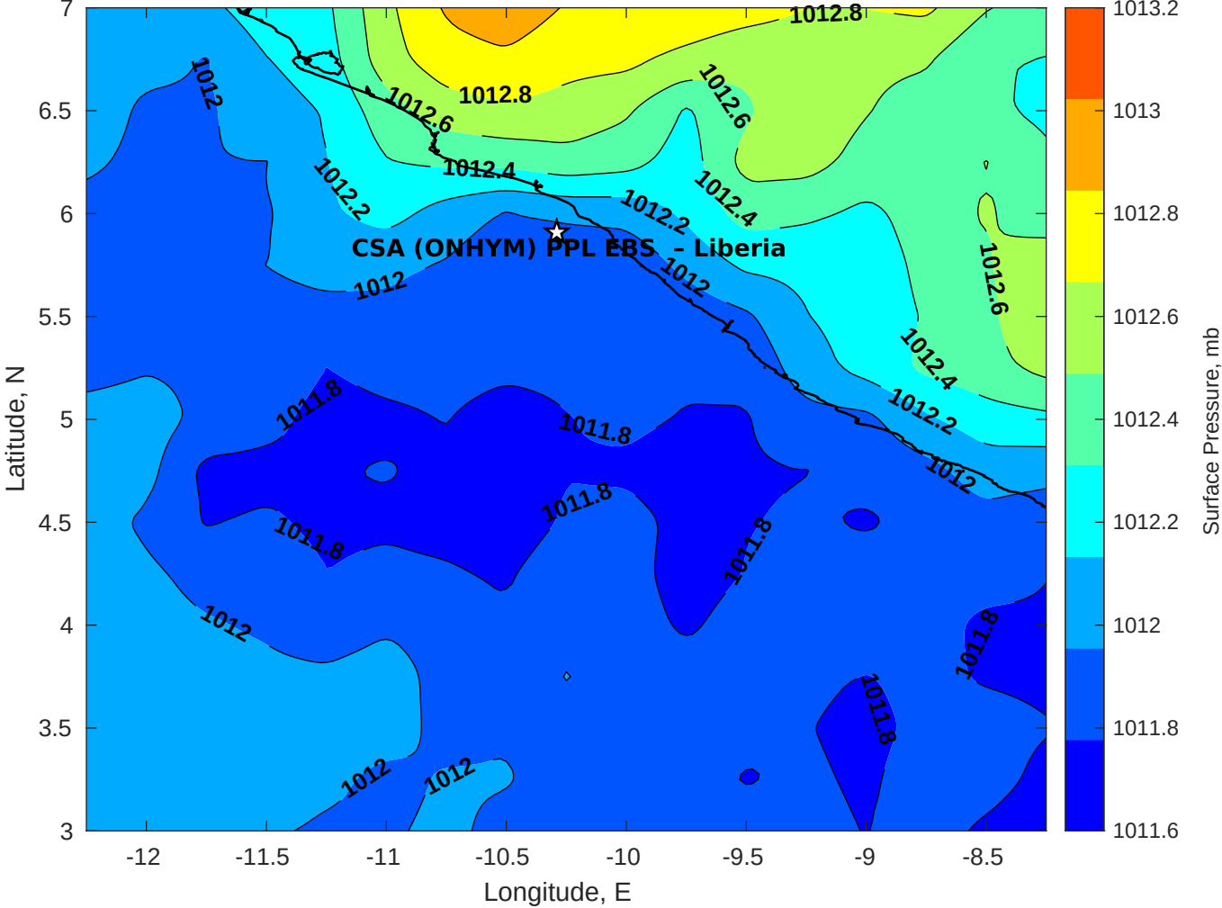
Surface Pressure (mb) for CSA (ONHYM) PPL EBS - Liberia at 15-Dec-2025 00:00:00
