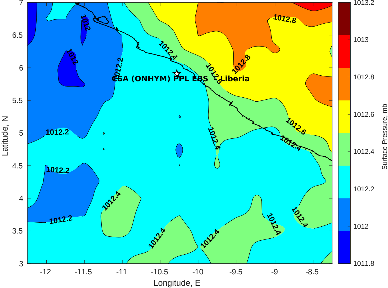
Surface Pressure (mb) for CSA (ONHYM) PPL EBS - Liberia at 16-Dec-2025 00:00:00
