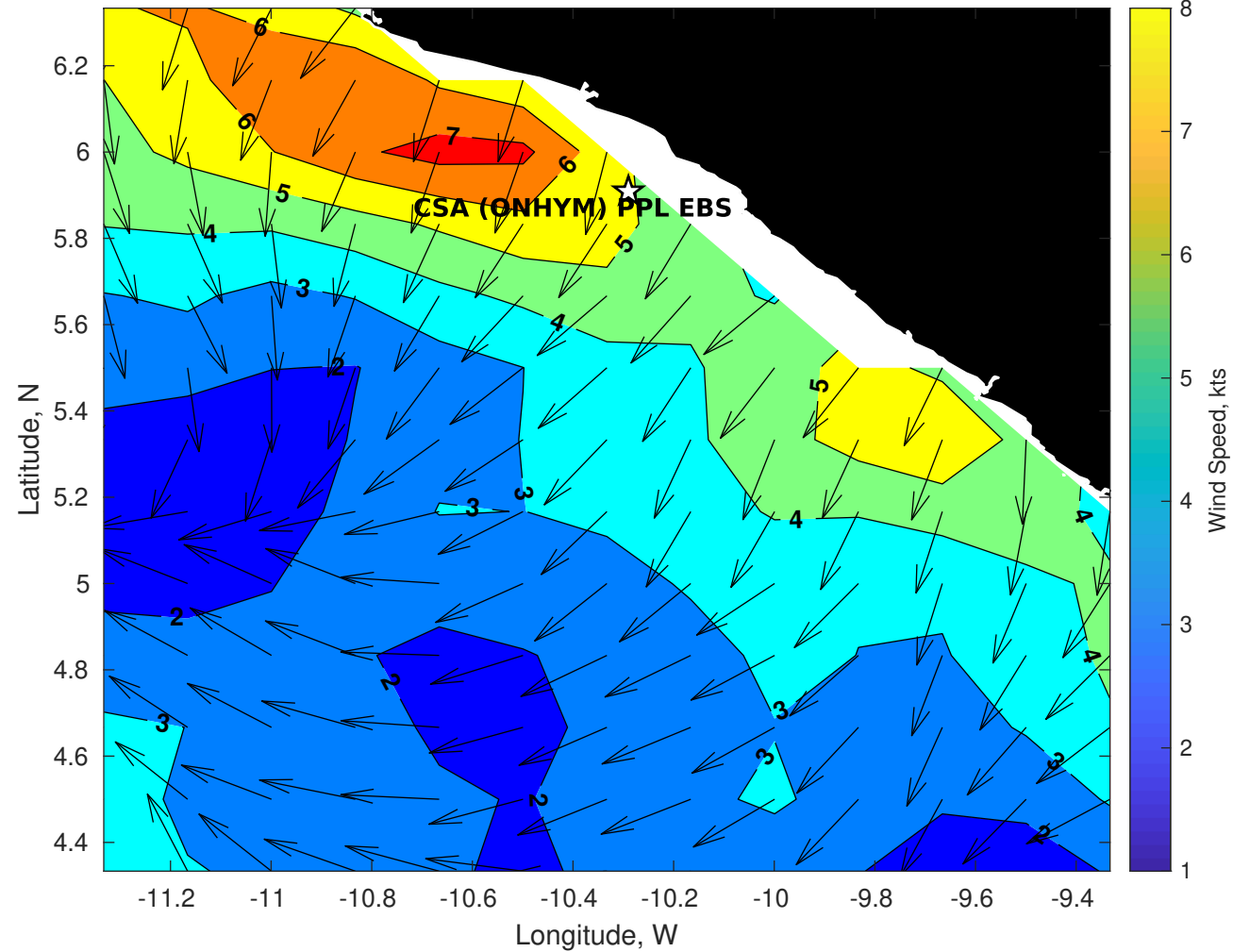
GFS Winds (kts) for CSA (ONHYM) PPL EBS - Liberia at 15-Dec-2025 09:00:00
