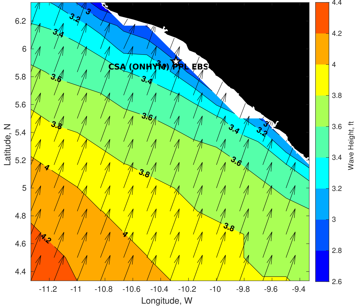
GFS Wave Height (ft) for CSA (ONHYM) PPL EBS - Liberia at 15-Dec-2025 09:00:00
