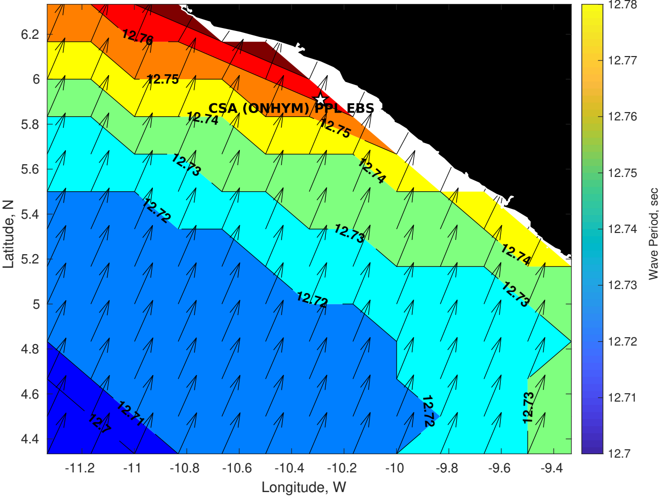
GFS Wave Period (sec) for CSA (ONHYM) PPL EBS - Liberia at 15-Dec-2025 09:00:00
