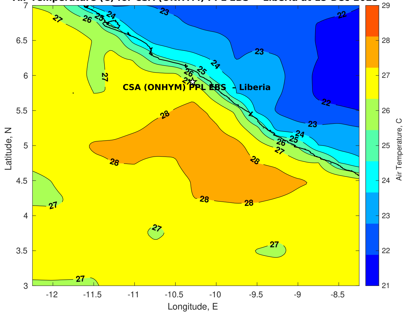
Air Temperature (C) for CSA (ONHYM) PPL EBS - Liberia at 15-Dec-2025
