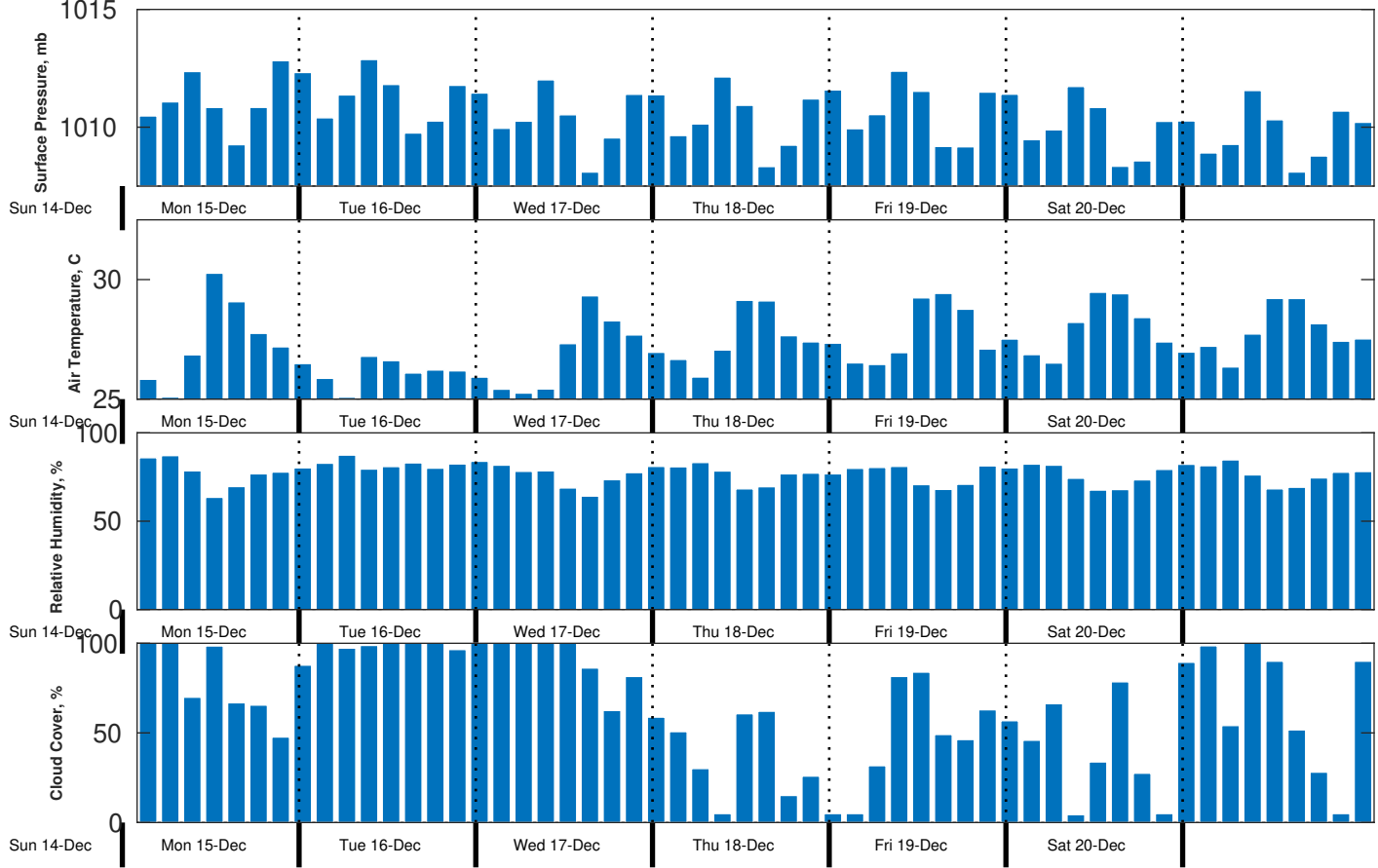
Met Forecast for CSA (ONHYM) PPL EBS - Liberia from 15-Dec-2025 00:00:00 to 22-Dec-2025 00:00:00
