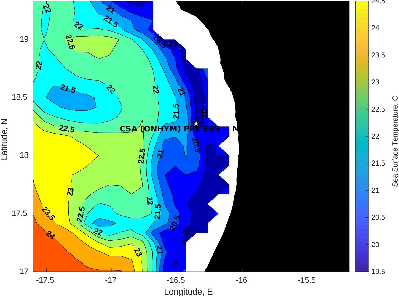
SST for CSA (ONHYM) PPL EBS - Mauritania at 14-Dec-2025 00:00:00
