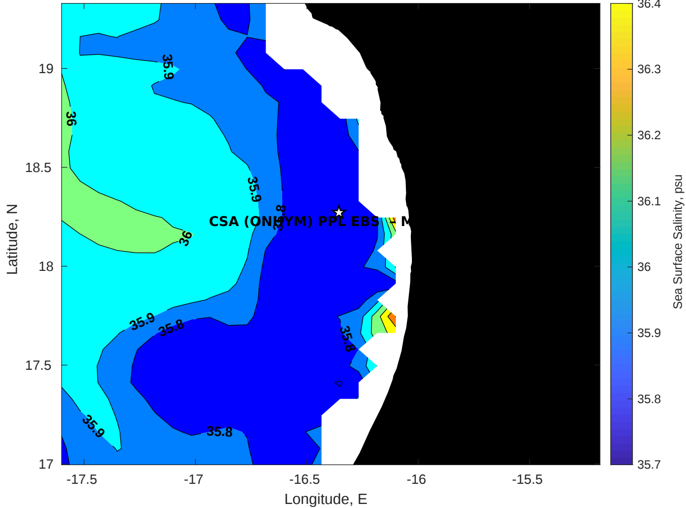
Surface Salinity for CSA (ONHYM) PPL EBS - Mauritania at 14-Dec-2025 00:00:00
