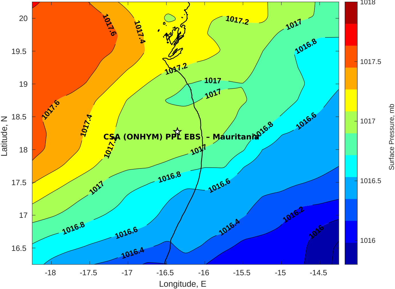
Surface Pressure (mb) for CSA (ONHYM) PPL EBS - Mauritania at 15-Dec-2025 00:00:00
