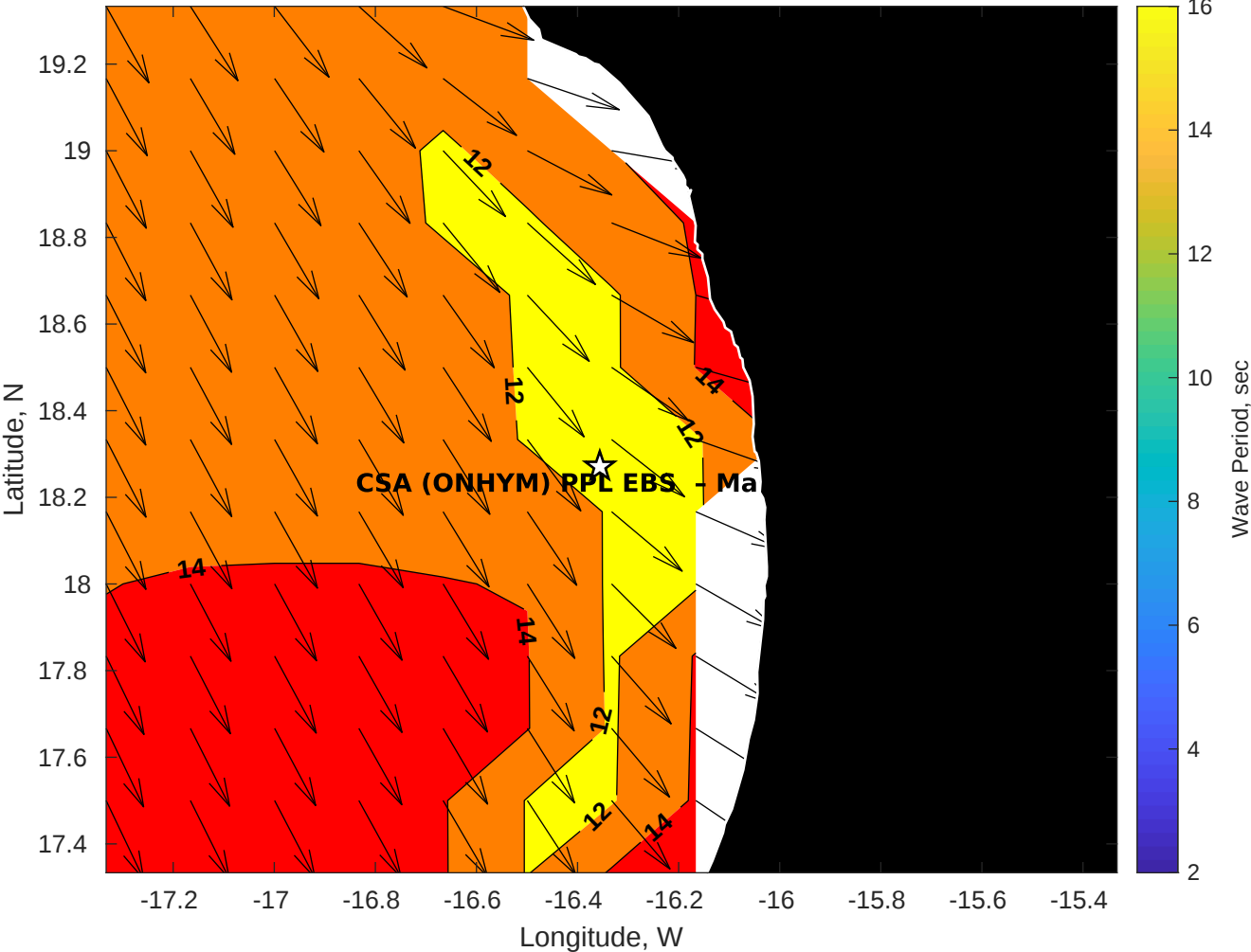
GFS Wave Period (sec) for CSA (ONHYM) PPL EBS - Mauritania at 15-Dec-2025 09:00:00
