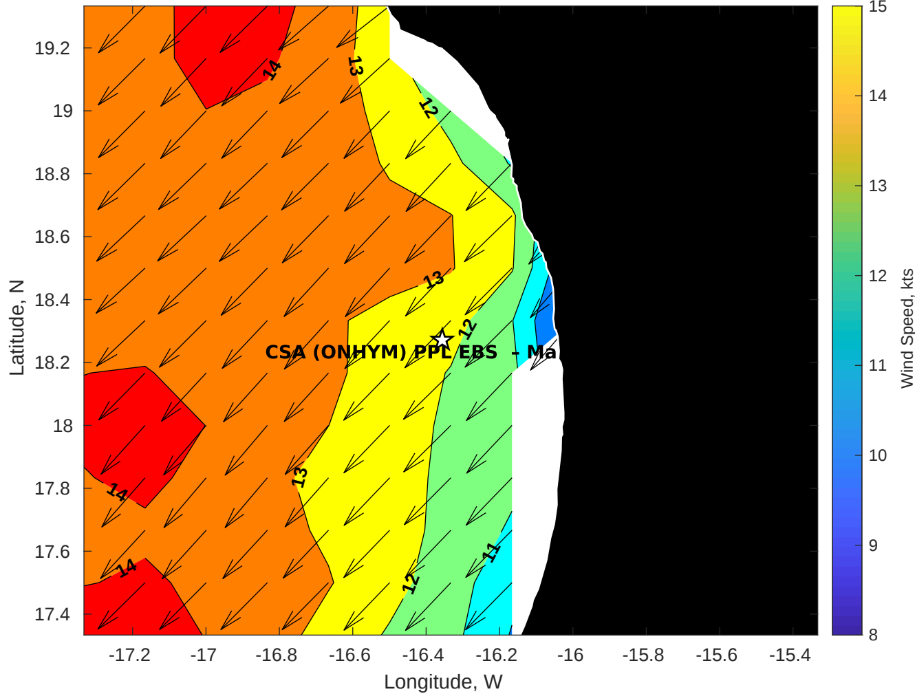
GFS Winds (kts) for CSA (ONHYM) PPL EBS - Mauritania at 15-Dec-2025 09:00:00
