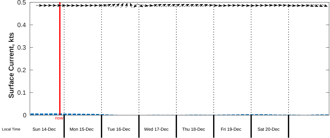
Surface Current Forecast for CSA (ONHYM) PPL EBS - Mauritania from 14-Dec-2025 00:00:00 to 22-Dec-2025 00:00:00
