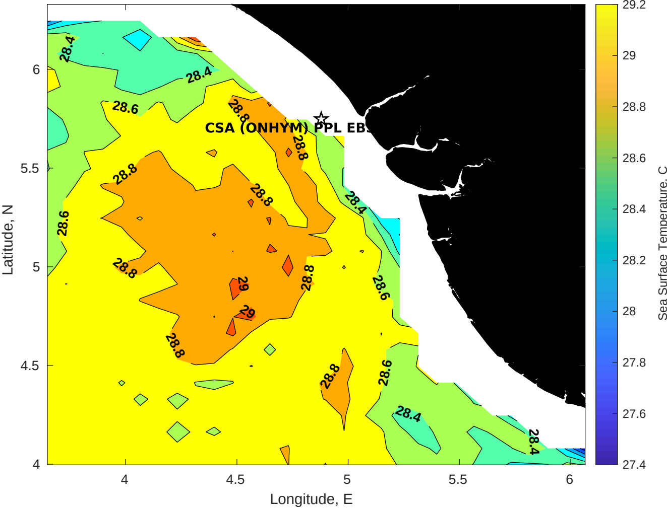
SST for CSA (ONHYM) PPL EBS - Nigeria at 14-Dec-2025 00:00:00
