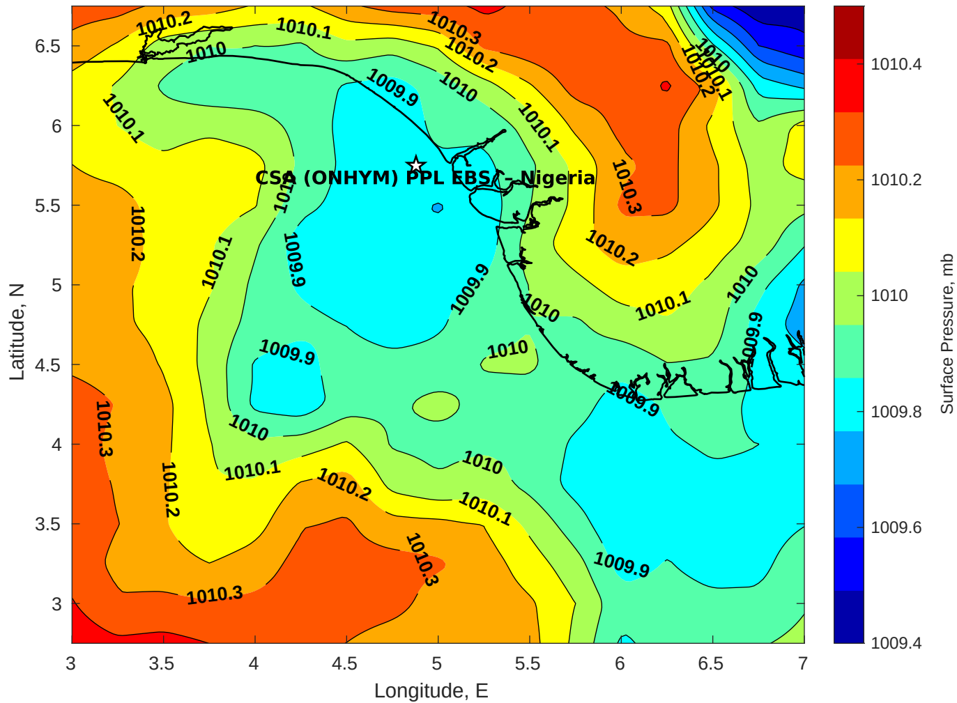
Surface Pressure (mb) for CSA (ONHYM) PPL EBS - Nigeria at 15-Dec-2025 00:00:00
