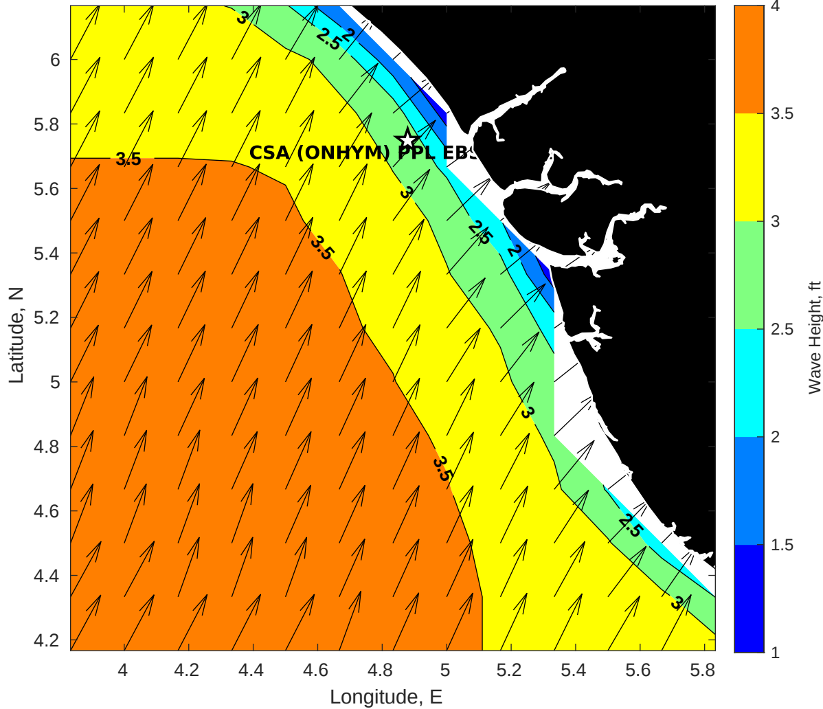
GFS Wave Height (ft) for CSA (ONHYM) PPL EBS - Nigeria at 15-Dec-2025 09:00:00
