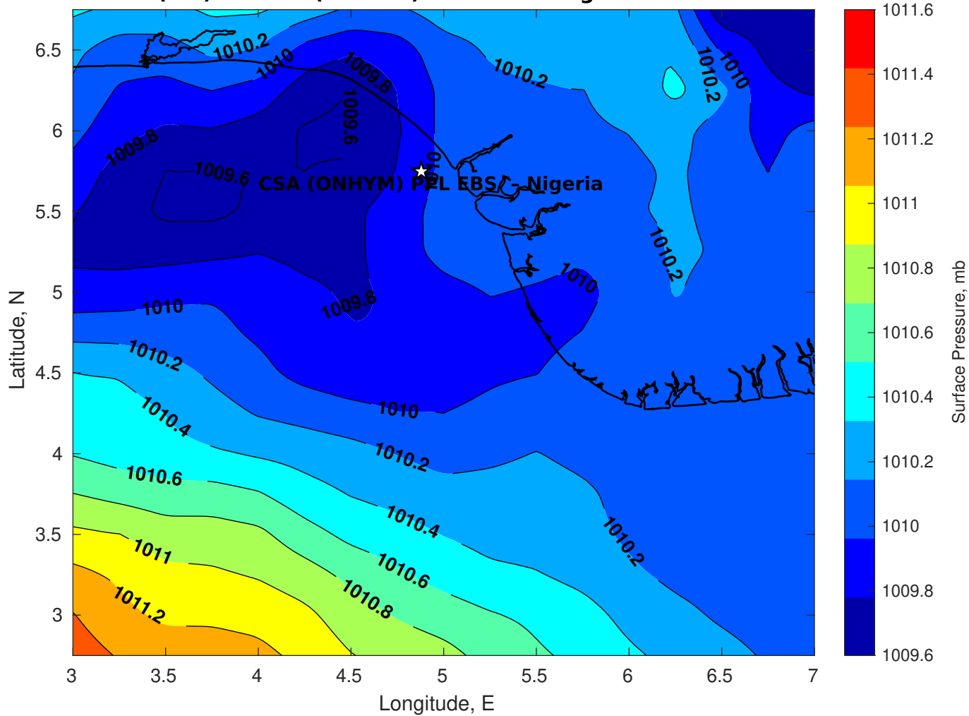
Surface Pressure (mb) for CSA (ONHYM) PPL EBS - Nigeria at 16-Dec-2025 00:00:00
