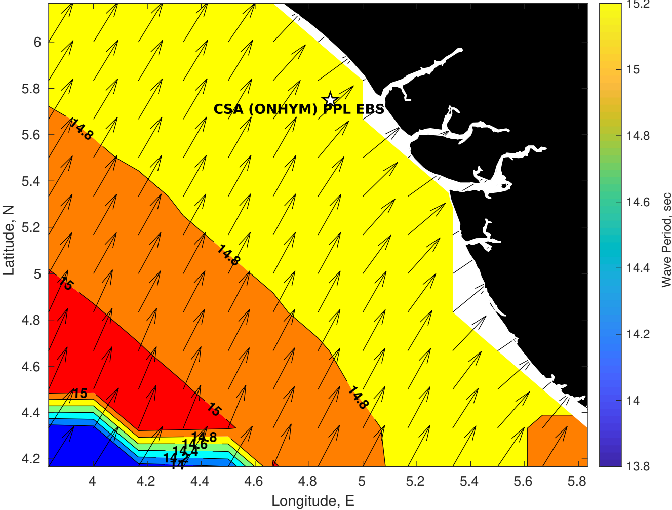
GFS Wave Period (sec) for CSA (ONHYM) PPL EBS - Nigeria at 15-Dec-2025 09:00:00
