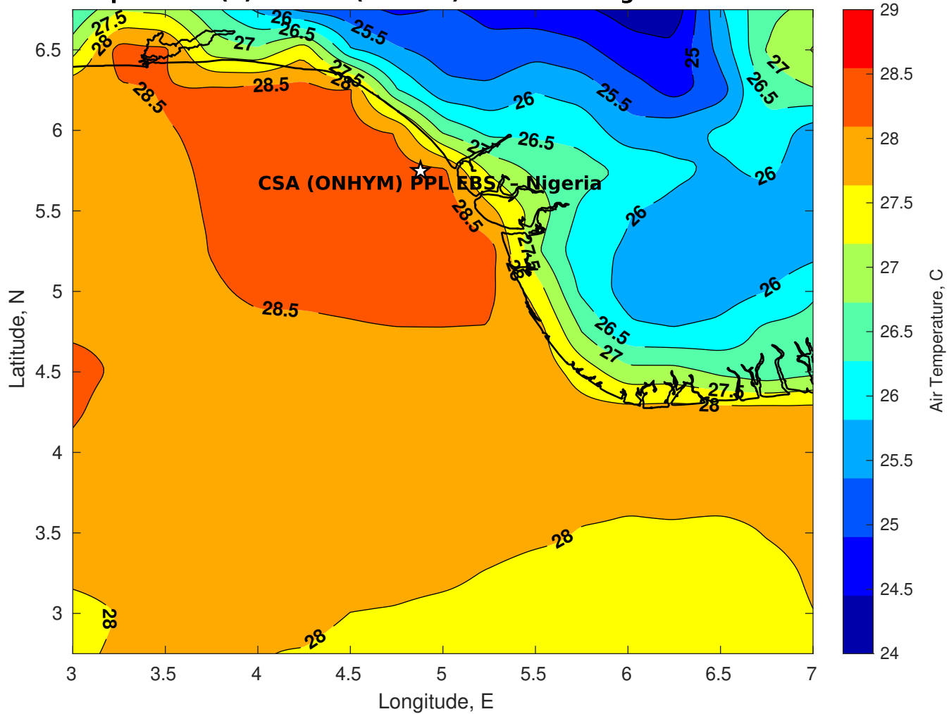
Air Temperature (C) for CSA (ONHYM) PPL EBS - Nigeria at 15-Dec-2025
