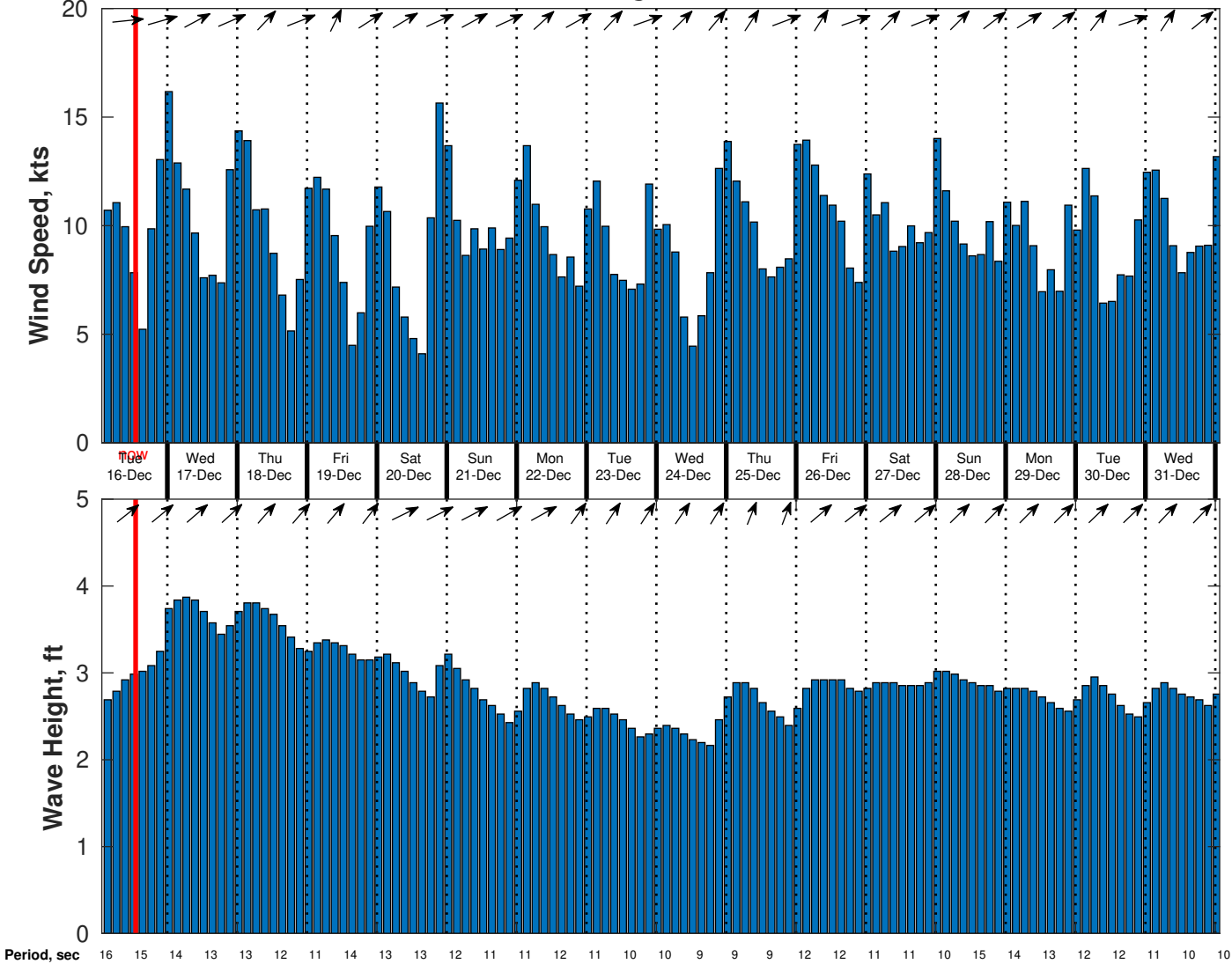
Wind & Wave Forecast for CSA (ONHYM) PPL EBS - Nigeria from 15-Dec-2025 02:00:00 to 31-Dec-2025 02:00:00
