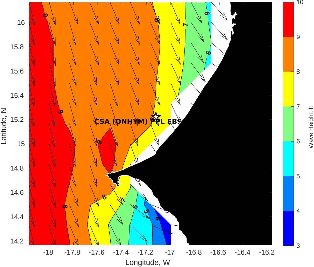
GFS Wave Height (ft) for CSA (ONHYM) PPL EBS - Senegal at 15-Dec-2025 09:00:00
