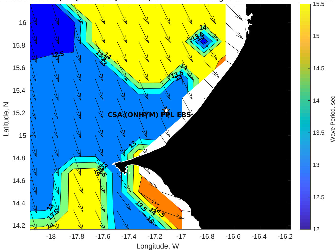
GFS Wave Period (sec) for CSA (ONHYM) PPL EBS - Senegal at 15-Dec-2025 09:00:00
