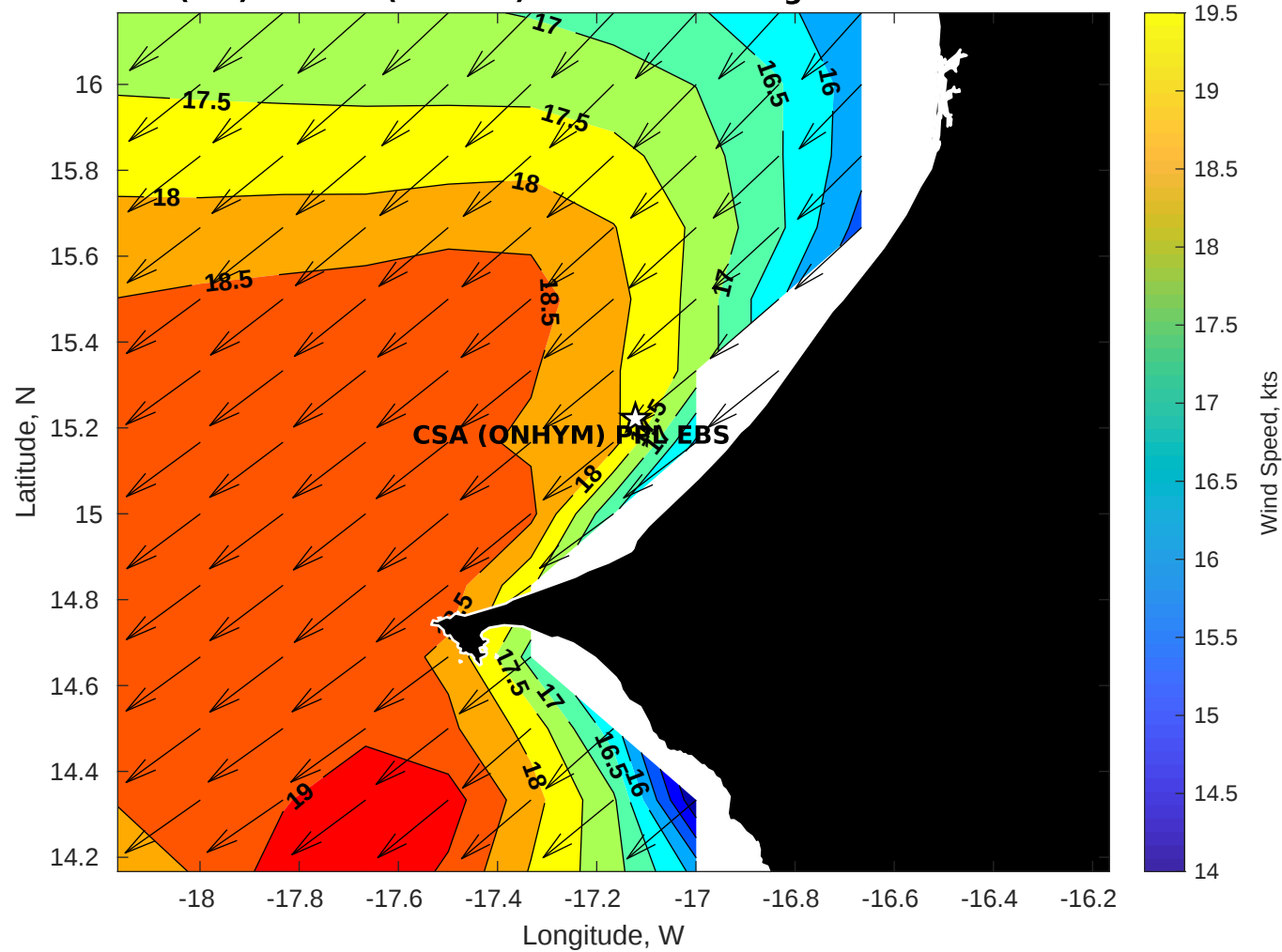
GFS Winds (kts) for CSA (ONHYM) PPL EBS - Senegal at 15-Dec-2025 09:00:00
