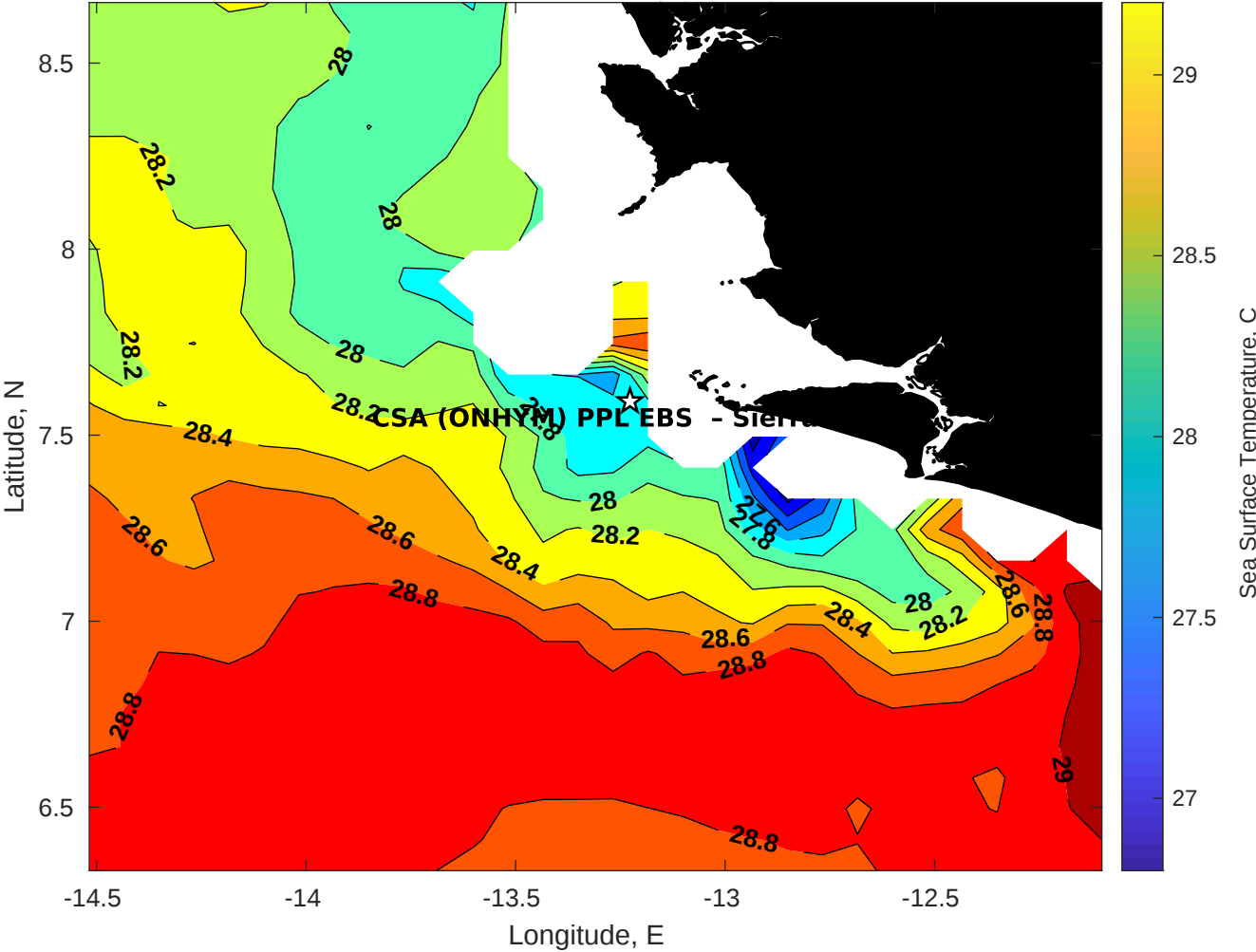
SST for CSA (ONHYM) PPL EBS - Sierra Leone at 14-Dec-2025 00:00:00
