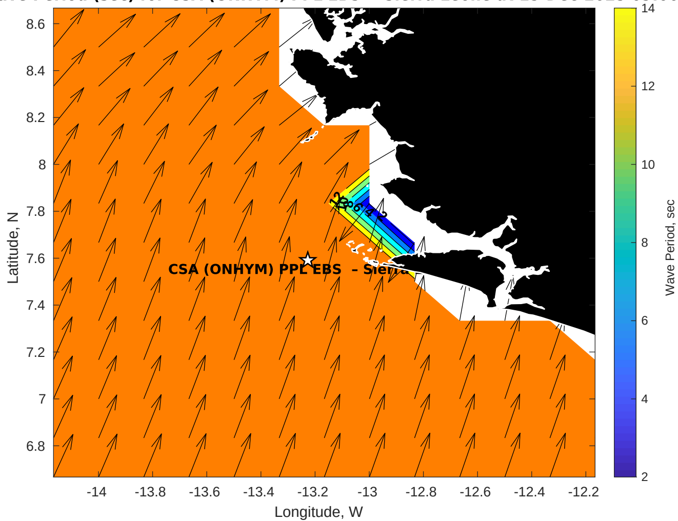
GFS Wave Period (sec) for CSA (ONHYM) PPL EBS - Sierra Leone at 15-Dec-2025 09:00:00
