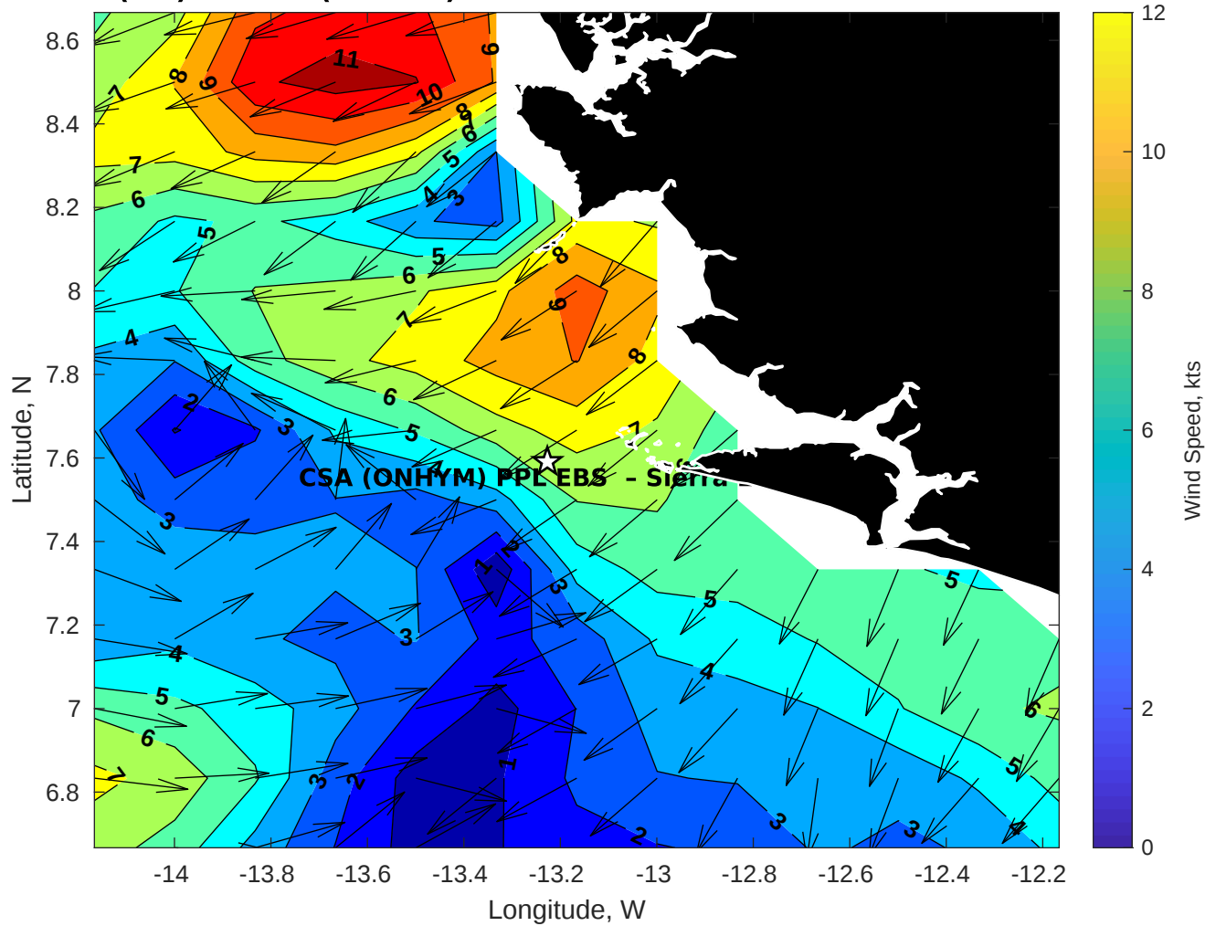
GFS Winds (kts) for CSA (ONHYM) PPL EBS - Sierra Leone at 15-Dec-2025 09:00:00
