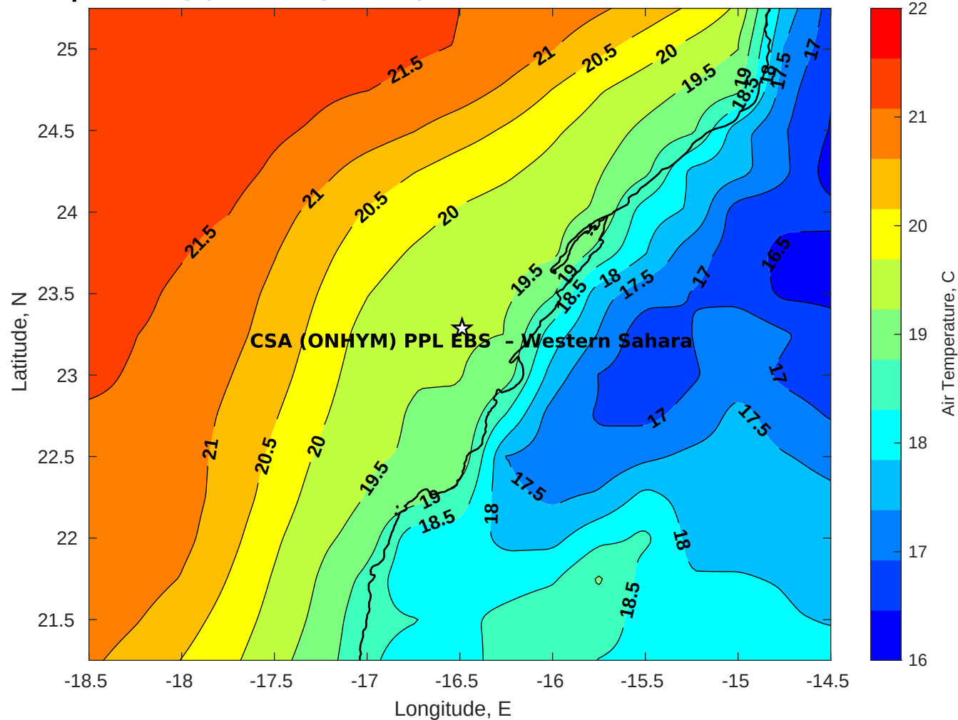
Air Temperature (C) for CSA (ONHYM) PPL EBS - Western Sahara at 15-Dec-2025
