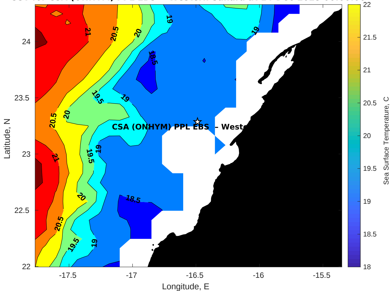
SST for CSA (ONHYM) PPL EBS - Western Sahara at 14-Dec-2025 00:00:00
