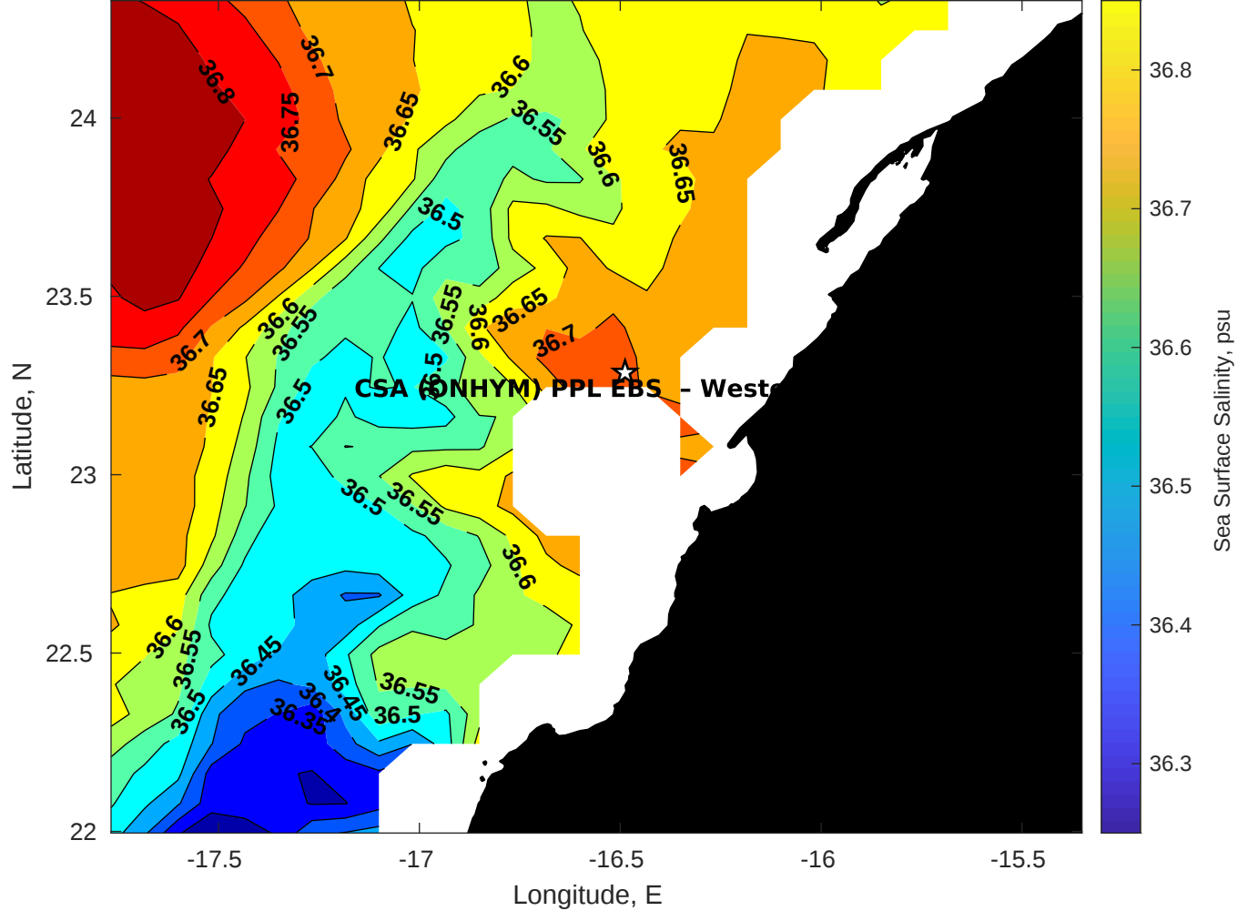
Surface Salinity for CSA (ONHYM) PPL EBS - Western Sahara at 14-Dec-2025 00:00:00
