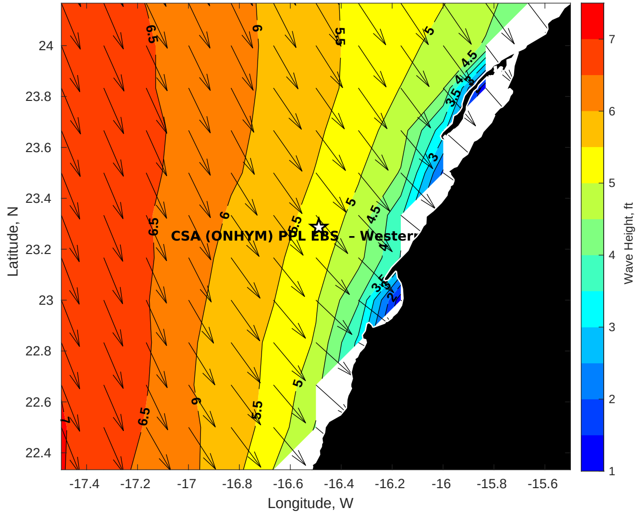
GFS Wave Height (ft) for CSA (ONHYM) PPL EBS - Western Sahara at 15-Dec-2025 09:00:00
