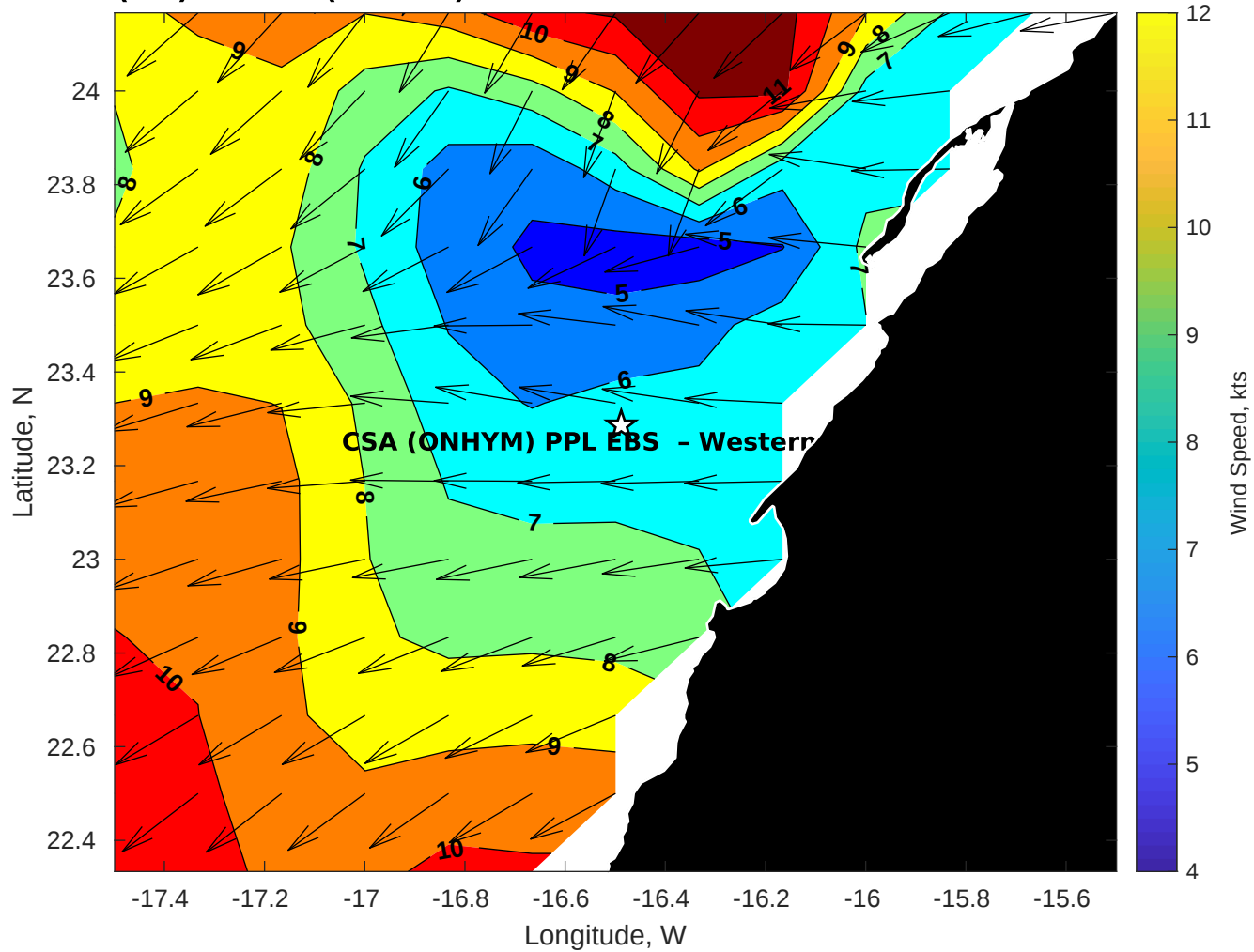
GFS Winds (kts) for CSA (ONHYM) PPL EBS - Western Sahara at 15-Dec-2025 09:00:00
