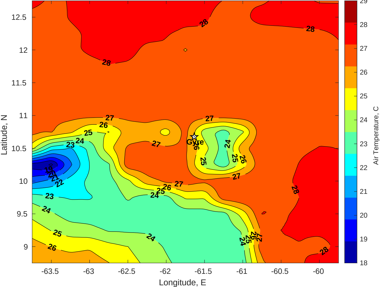
Air Temperature (C) for Gyre at 15-Dec-2025
