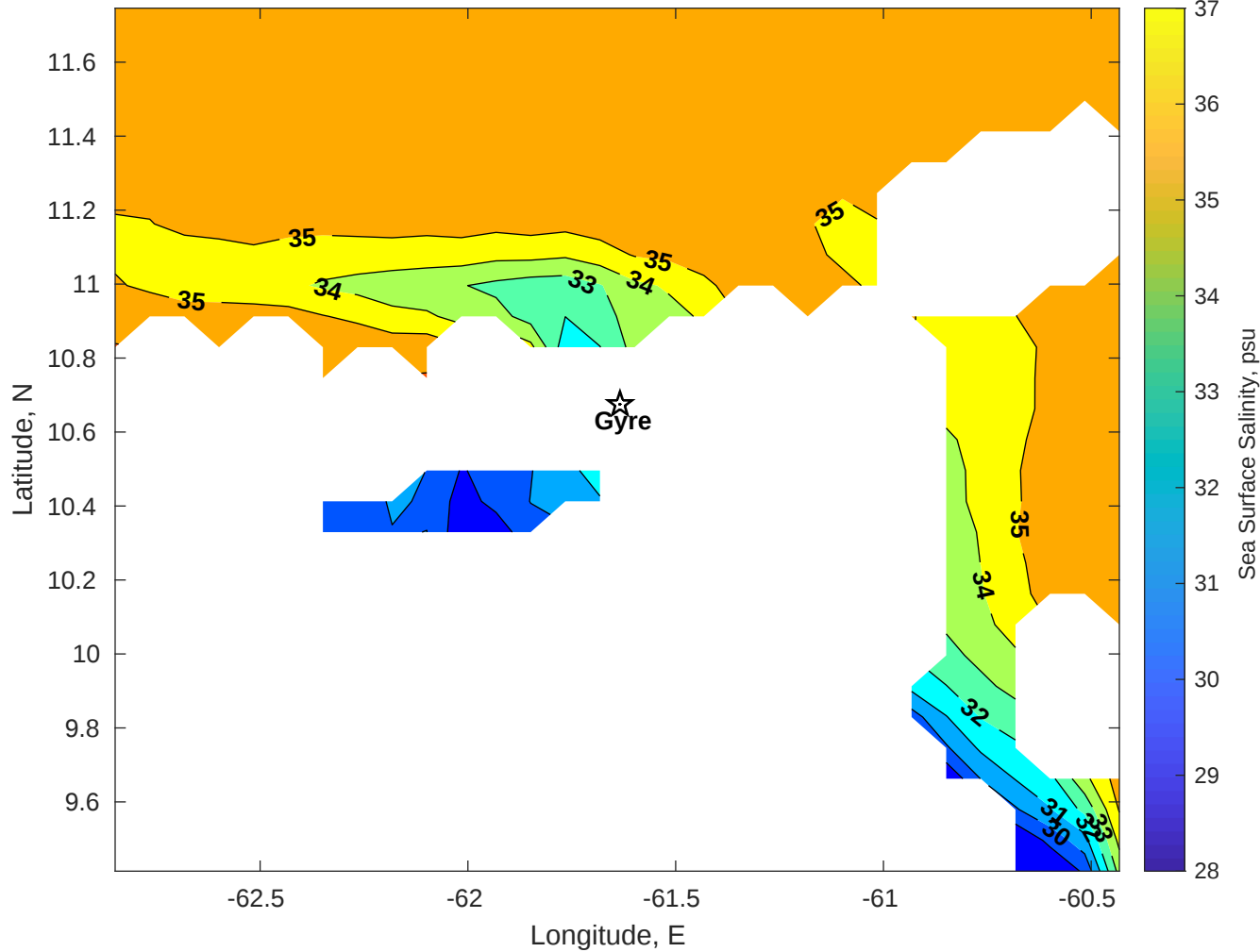
Surface Salinity for Gyre at 14-Dec-2025 00:00:00
