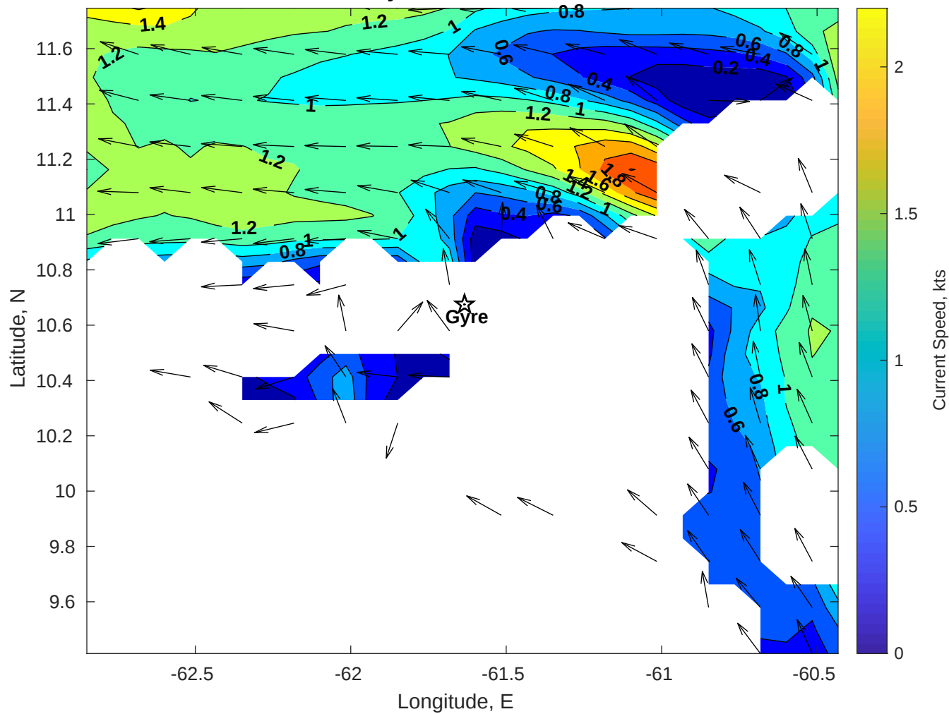
Surface Currents for Gyre at 14-Dec-2025 00:00:00
