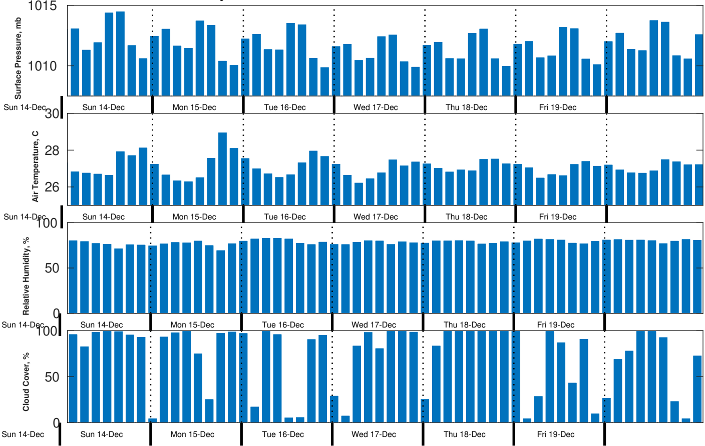
Met Forecast for Gyre from 14-Dec-2025 20:00:00 to 21-Dec-2025 20:00:00
