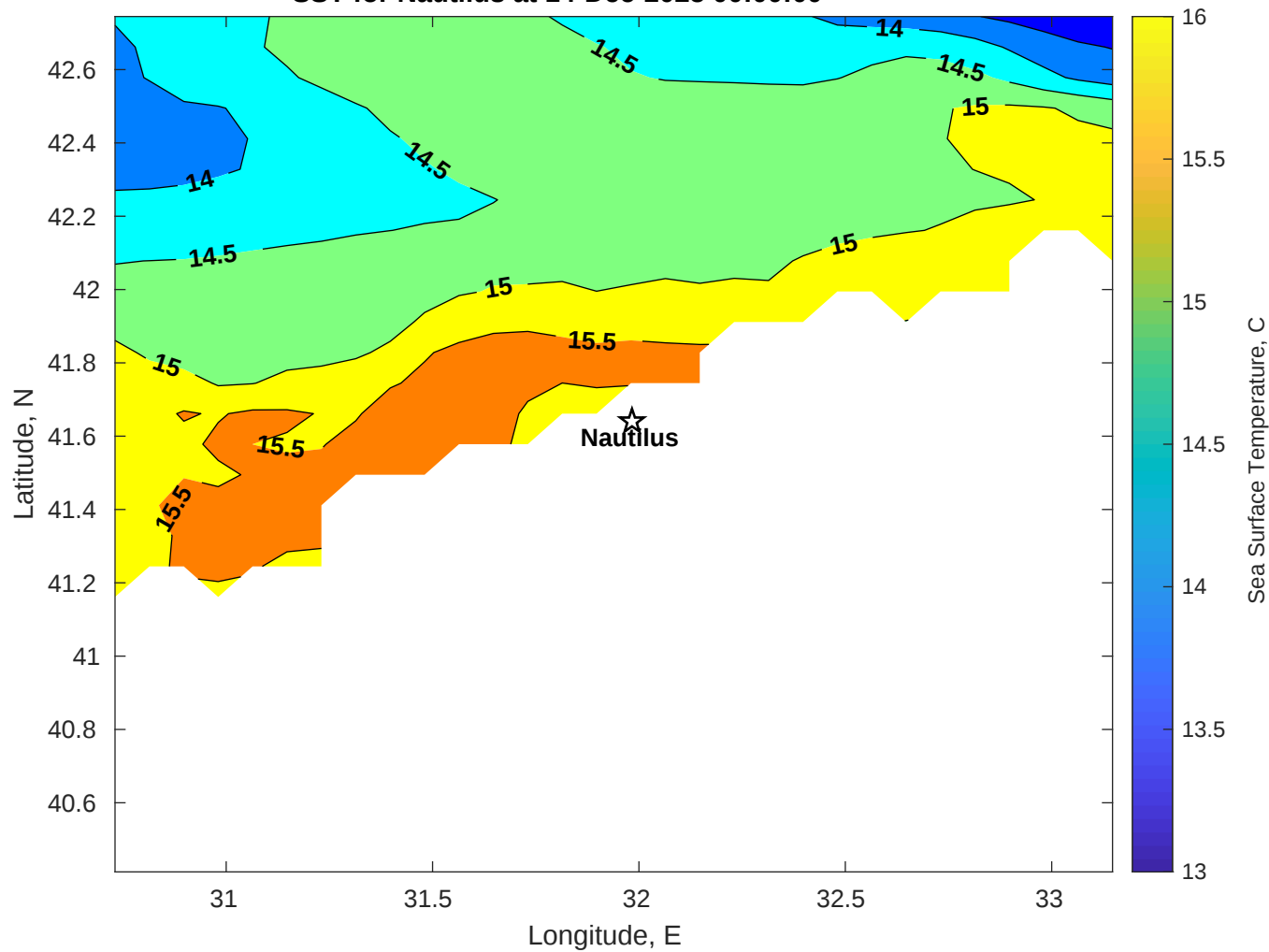
SST for Nautilus at 14-Dec-2025 00:00:00
