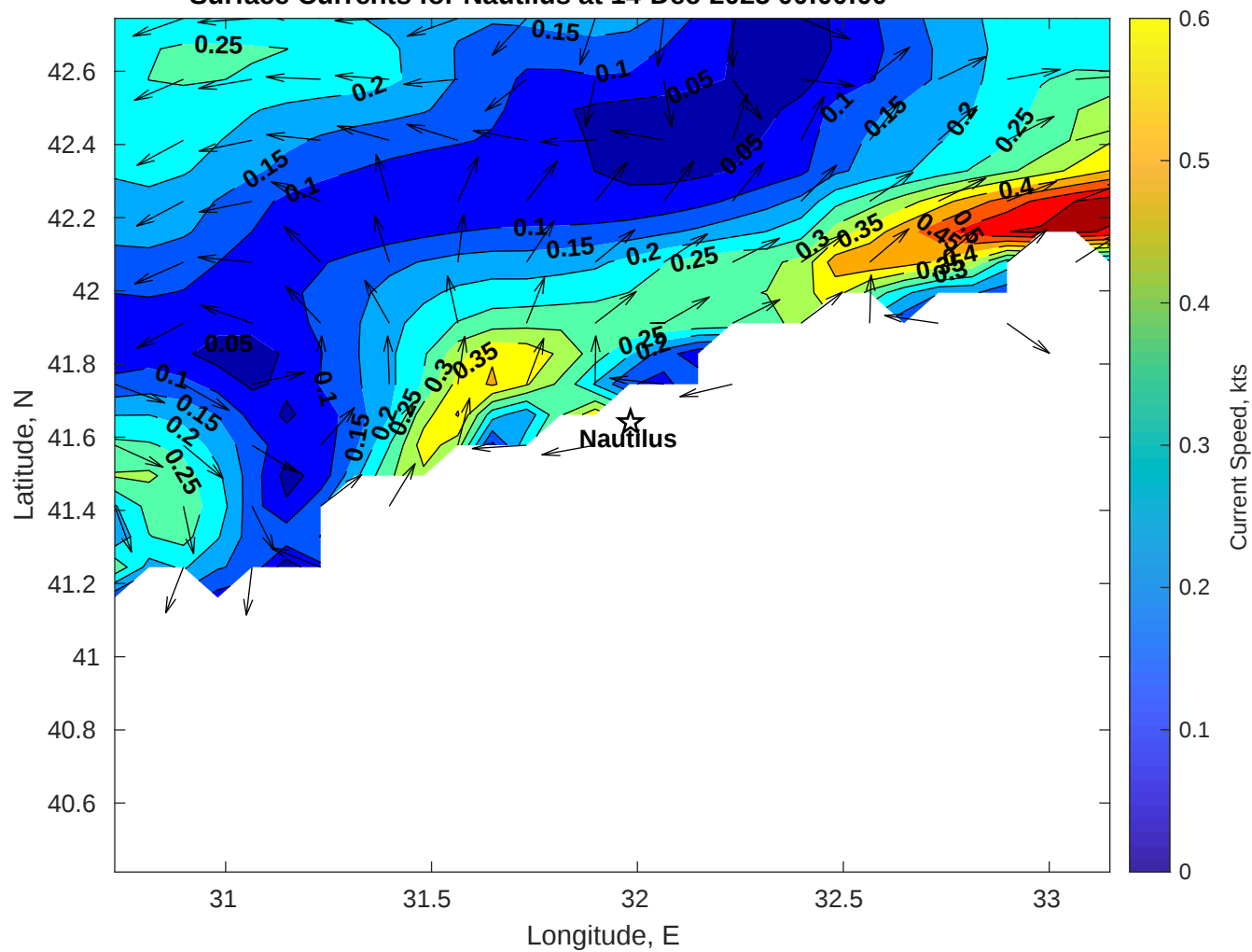
Surface Currents for Nautilus at 14-Dec-2025 00:00:00
