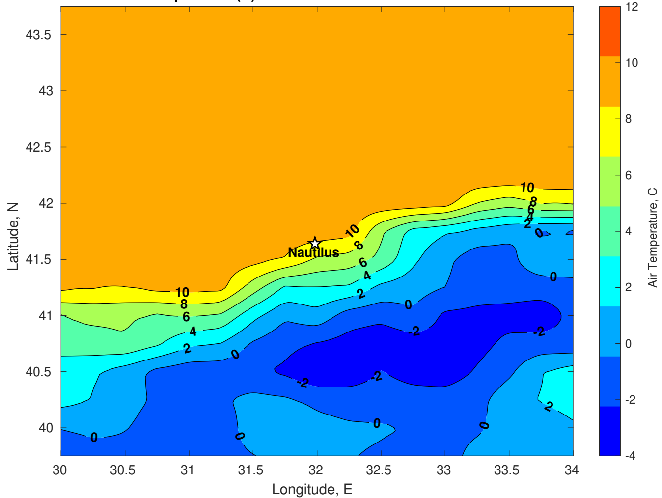
Air Temperature (C) for Nautilus at 15-Dec-2025
