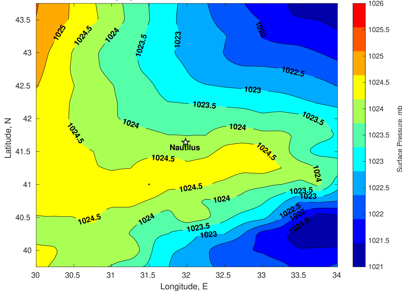
Surface Pressure (mb) for Nautilus at 15-Dec-2025 00:00:00
