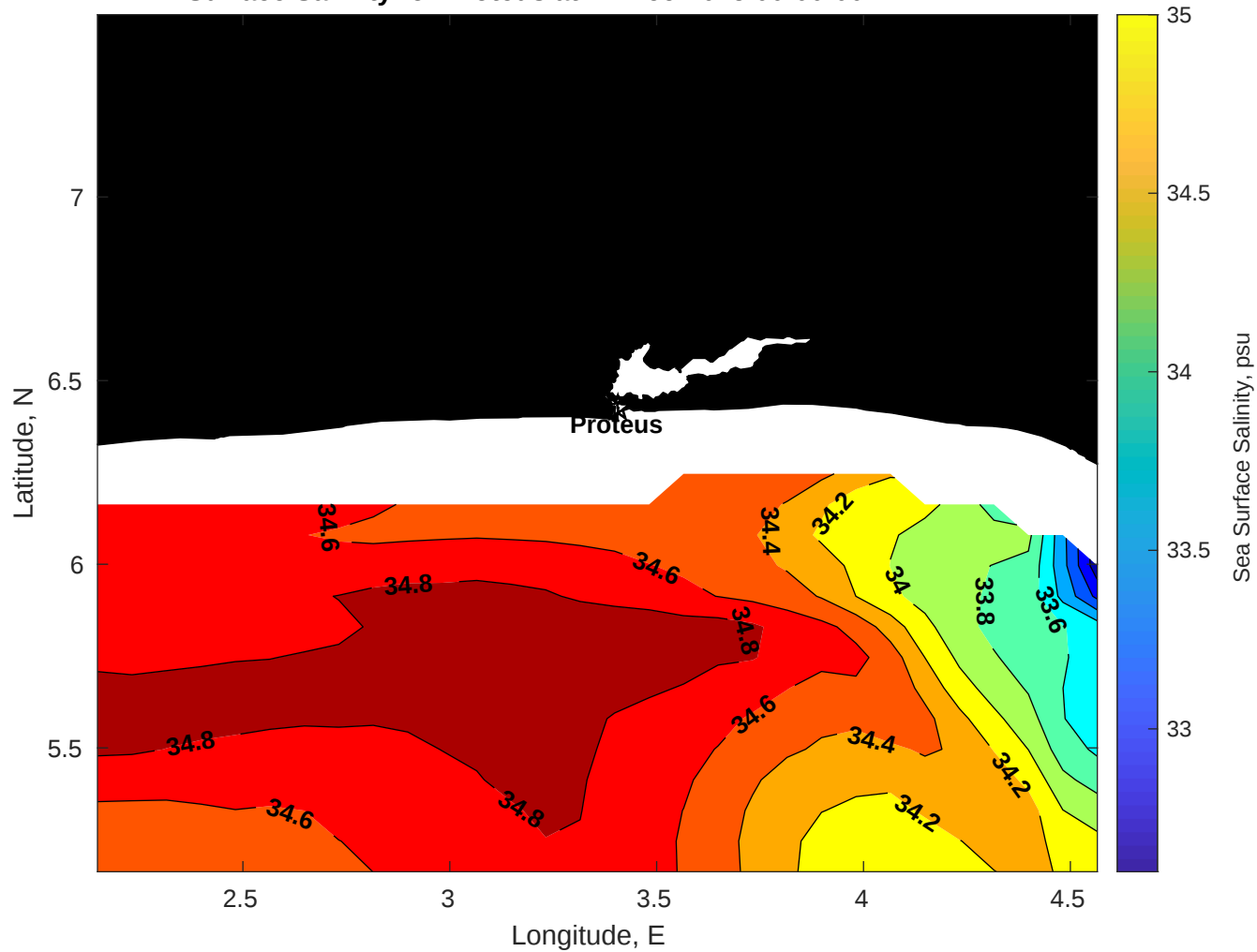
Surface Salinity for Proteus at 14-Dec-2025 00:00:00
