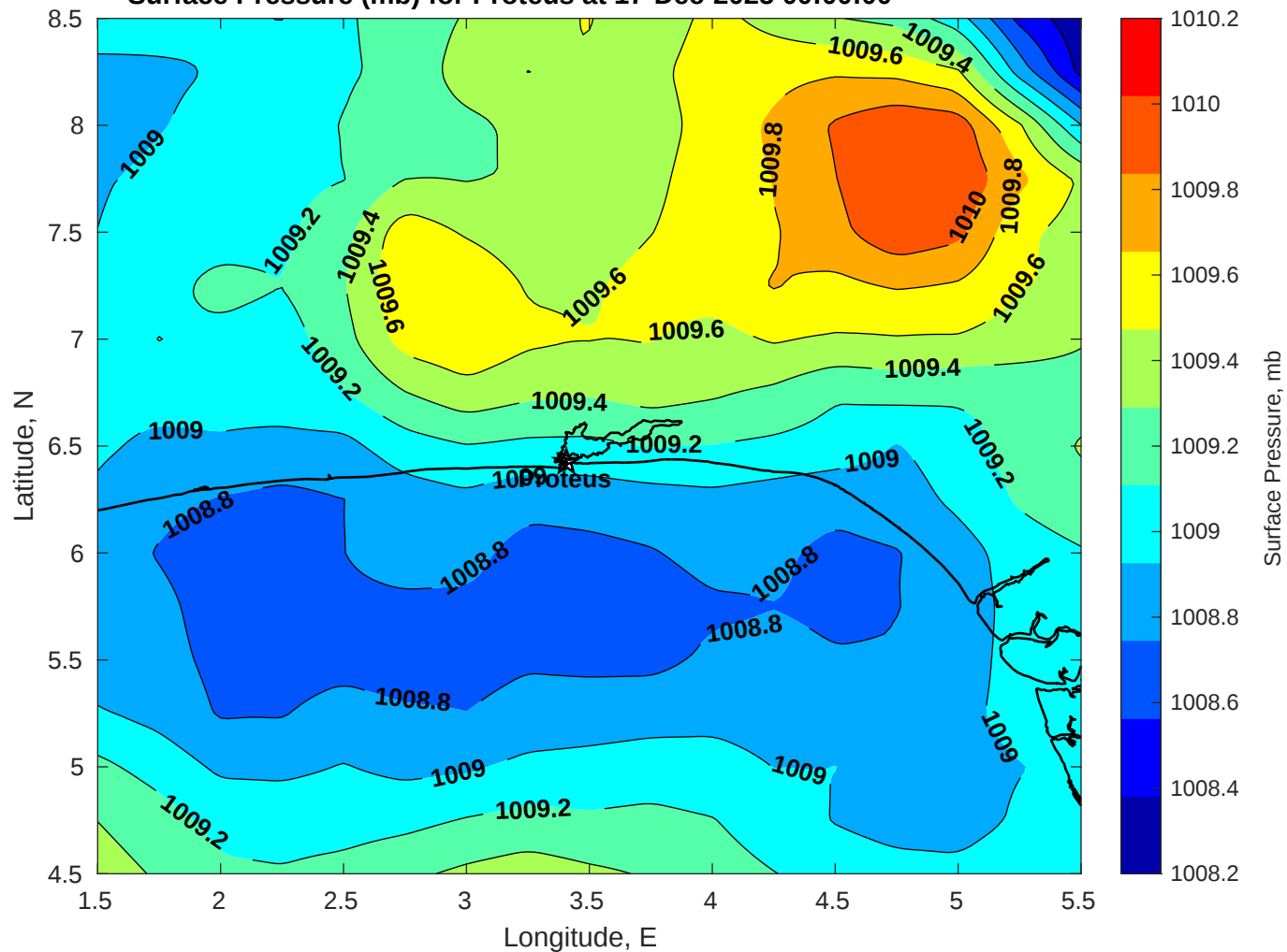
Surface Pressure (mb) for Proteus at 17-Dec-2025 00:00:00
