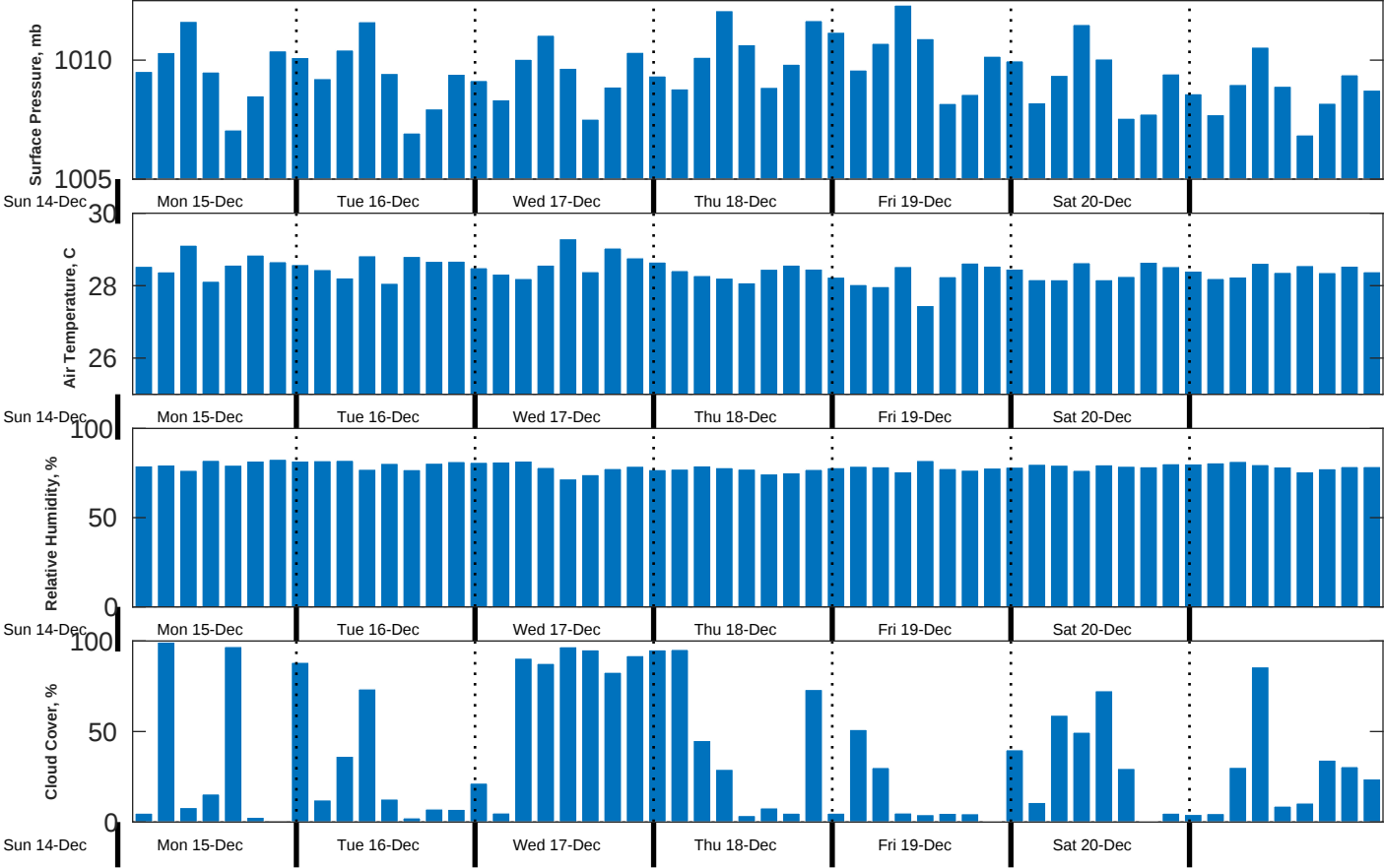
Met Forecast for Proteus from 15-Dec-2025 00:00:00 to 22-Dec-2025 00:00:00
